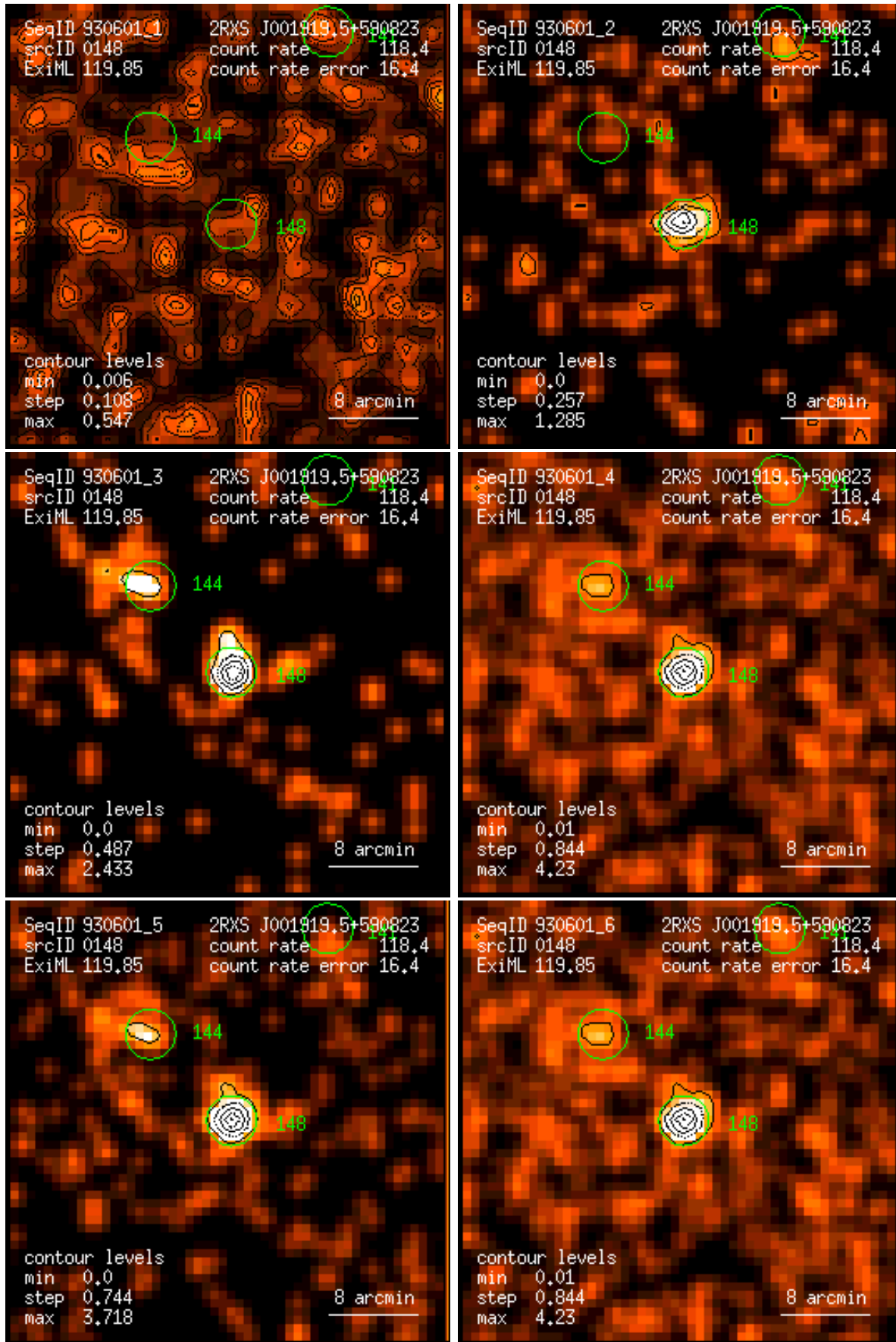
Figure 148: RASS 930601: detection 0148: band rate images, Gaussian filter: (1) PSPC channels 11 – 41, (2) 52 – 90, (3) 91 – 201, (4) 11 – 235, (5) 52 – 201, (6) 11 – 201. Broad band rates in counts/ks. Band rate contour levels in counts/ks/arcmin 2 .
