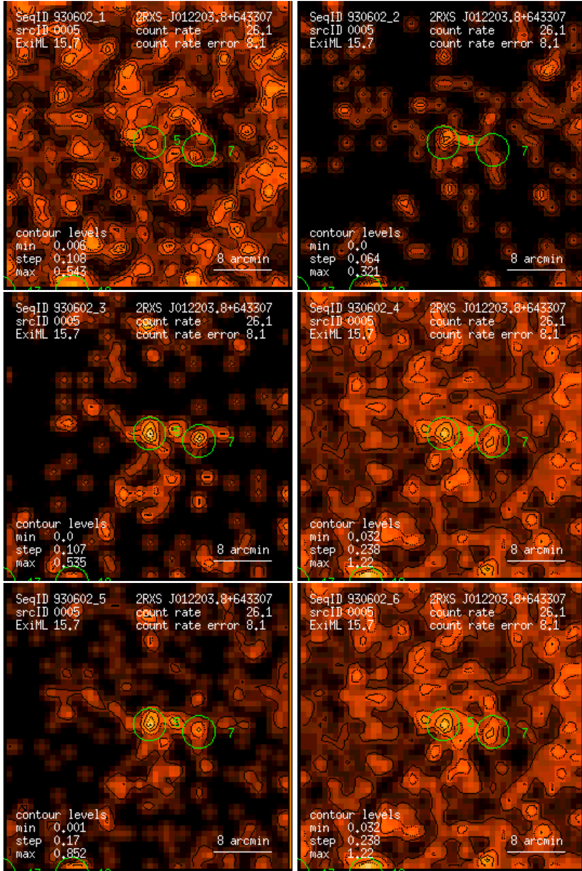
Figure 5: RASS 930602: detection 0005: band rate images, Gaussian filter: (1) PSPC channels 11 – 41, (2) 52 – 90, (3) 91 – 201, (4) 11 – 235, (5) 52 – 201, (6) 11 – 201. Broad band rates in counts/ks. Band rate contour levels in counts/ks/arcmin 2 .
