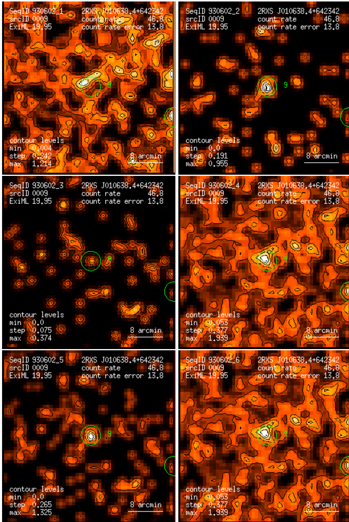
Figure 9: RASS 930602: detection 0009: band rate images, Gaussian filter: (1) PSPC channels 11 – 41, (2) 52 – 90, (3) 91 – 201, (4) 11 – 235, (5) 52 – 201, (6) 11 – 201. Broad band rates in counts/ks. Band rate contour levels in counts/ks/arcmin 2 .
