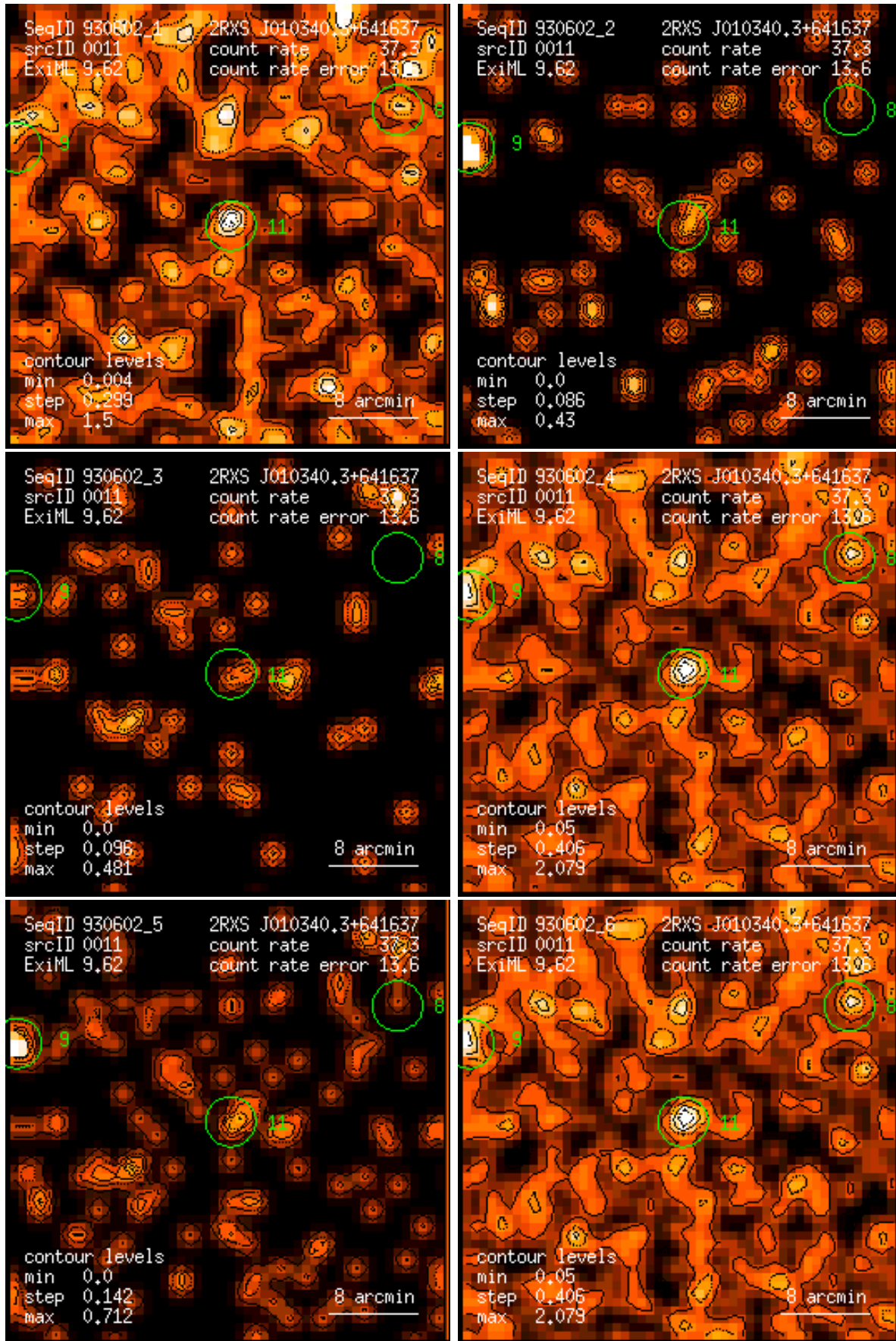
Figure 11: RASS 930602: detection 0011: band rate images, Gaussian filter: (1) PSPC channels 11 – 41, (2) 52 – 90, (3) 91 – 201, (4) 11 – 235, (5) 52 – 201, (6) 11 – 201. Broad band rates in counts/ks. Band rate contour levels in counts/ks/arcmin 2 .
