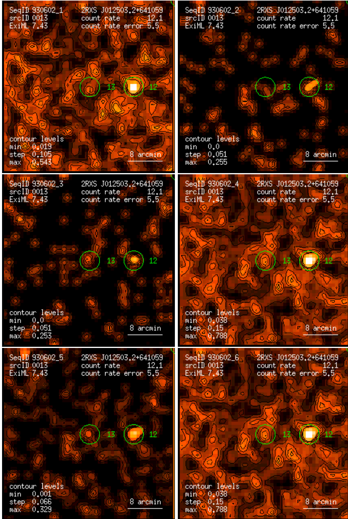
Figure 13: RASS 930602: detection 0013: band rate images, Gaussian filter: (1) PSPC channels 11 – 41, (2) 52 – 90, (3) 91 – 201, (4) 11 – 235, (5) 52 – 201, (6) 11 – 201. Broad band rates in counts/ks. Band rate contour levels in counts/ks/arcmin 2 .
