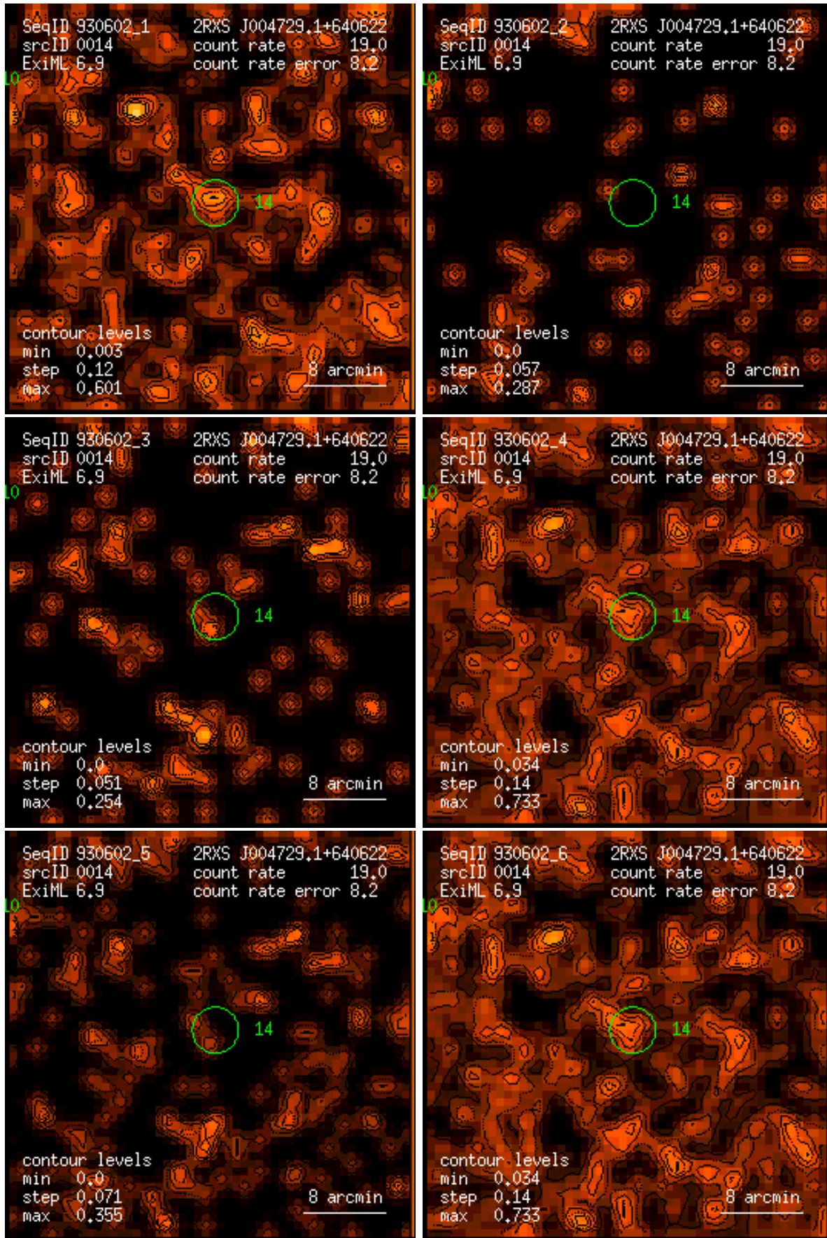
Figure 14: RASS 930602: detection 0014: band rate images, Gaussian filter: (1) PSPC channels 11 – 41, (2) 52 – 90, (3) 91 – 201, (4) 11 – 235, (5) 52 – 201, (6) 11 – 201. Broad band rates in counts/ks. Band rate contour levels in counts/ks/arcmin 2 .
