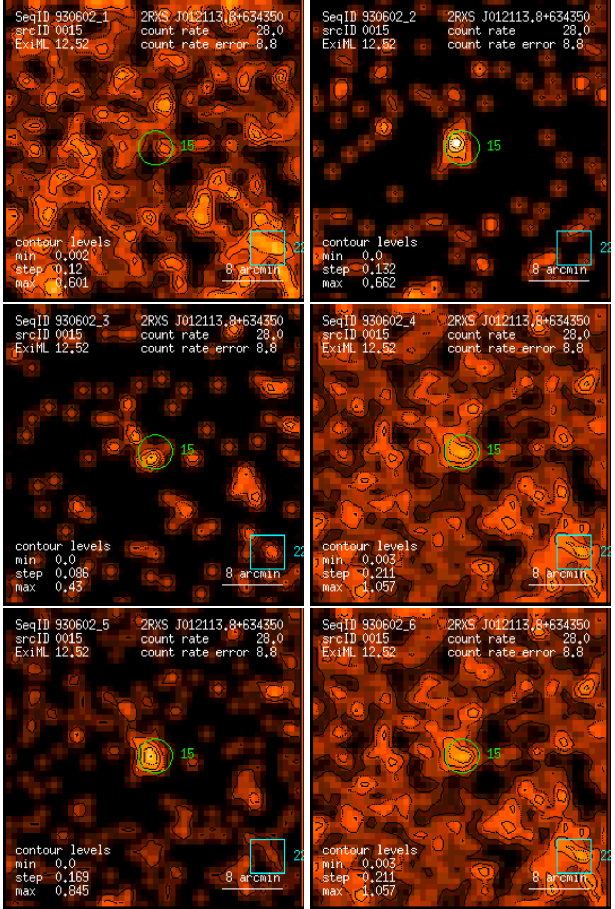
Figure 15: RASS 930602: detection 0015: band rate images, Gaussian filter: (1) PSPC channels 11 – 41, (2) 52 – 90, (3) 91 – 201, (4) 11 – 235, (5) 52 – 201, (6) 11 – 201. Broad band rates in counts/ks. Band rate contour levels in counts/ks/arcmin 2 .
