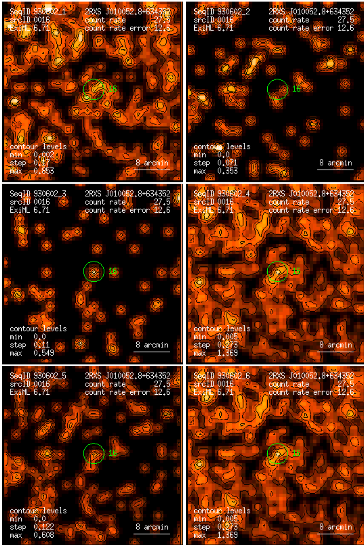
Figure 16: RASS 930602: detection 0016: band rate images, Gaussian filter: (1) PSPC channels 11 – 41, (2) 52 – 90, (3) 91 – 201, (4) 11 – 235, (5) 52 – 201, (6) 11 – 201. Broad band rates in counts/ks. Band rate contour levels in counts/ks/arcmin 2 .
