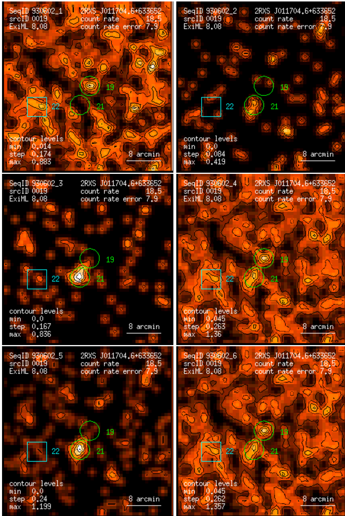
Figure 19: RASS 930602: detection 0019: band rate images, Gaussian filter: (1) PSPC channels 11 – 41, (2) 52 – 90, (3) 91 – 201, (4) 11 – 235, (5) 52 – 201, (6) 11 – 201. Broad band rates in counts/ks. Band rate contour levels in counts/ks/arcmin 2 .
