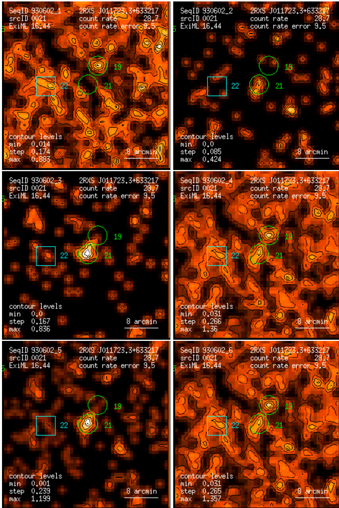
Figure 21: RASS 930602: detection 0021: band rate images, Gaussian filter: (1) PSPC channels 11 – 41, (2) 52 – 90, (3) 91 – 201, (4) 11 – 235, (5) 52 – 201, (6) 11 – 201. Broad band rates in counts/ks. Band rate contour levels in counts/ks/arcmin 2 .
