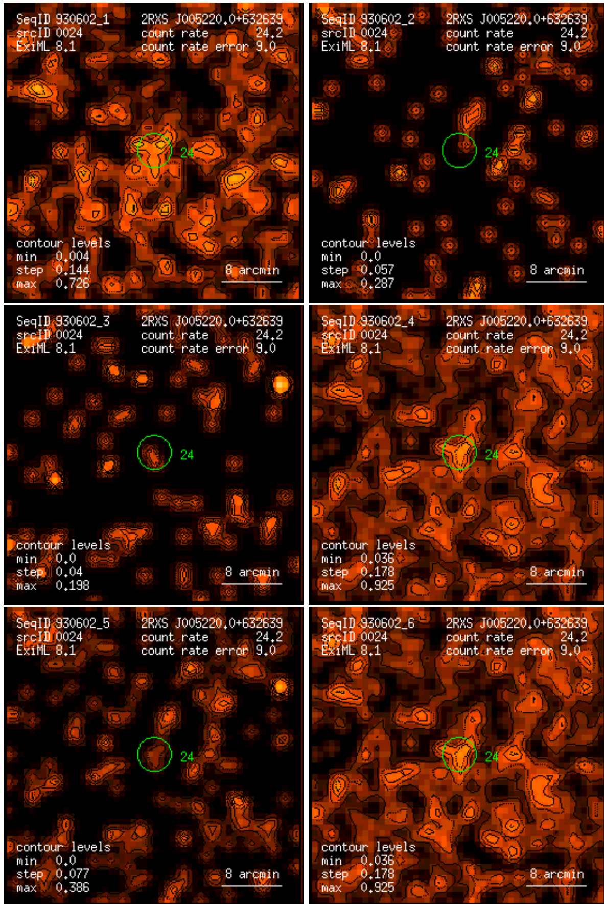
Figure 24: RASS 930602: detection 0024: band rate images, Gaussian filter: (1) PSPC channels 11 – 41, (2) 52 – 90, (3) 91 – 201, (4) 11 – 235, (5) 52 – 201, (6) 11 – 201. Broad band rates in counts/ks. Band rate contour levels in counts/ks/arcmin 2 .
