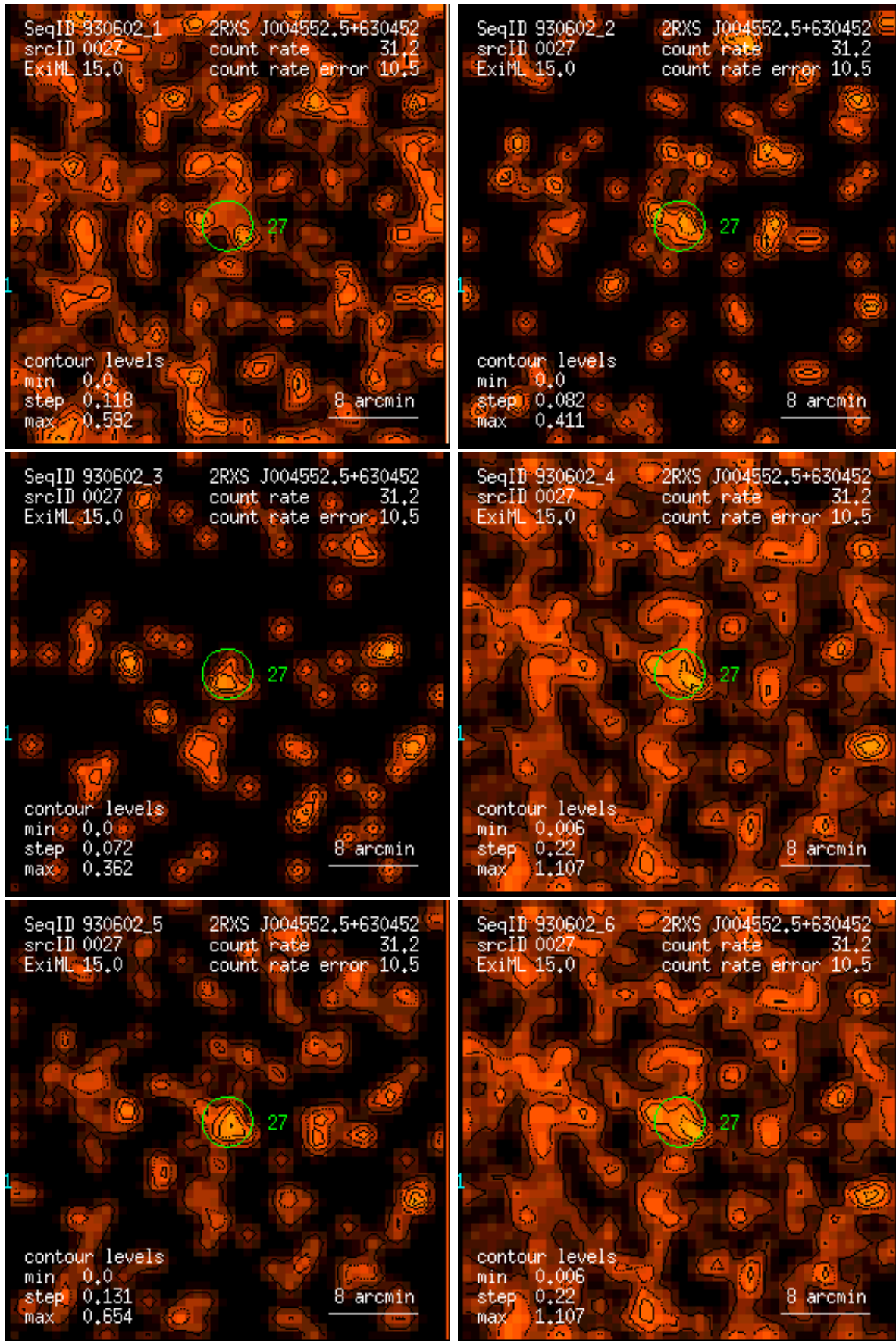
Figure 27: RASS 930602: detection 0027: band rate images, Gaussian filter: (1) PSPC channels 11 – 41, (2) 52 – 90, (3) 91 – 201, (4) 11 – 235, (5) 52 – 201, (6) 11 – 201. Broad band rates in counts/ks. Band rate contour levels in counts/ks/arcmin 2 .
