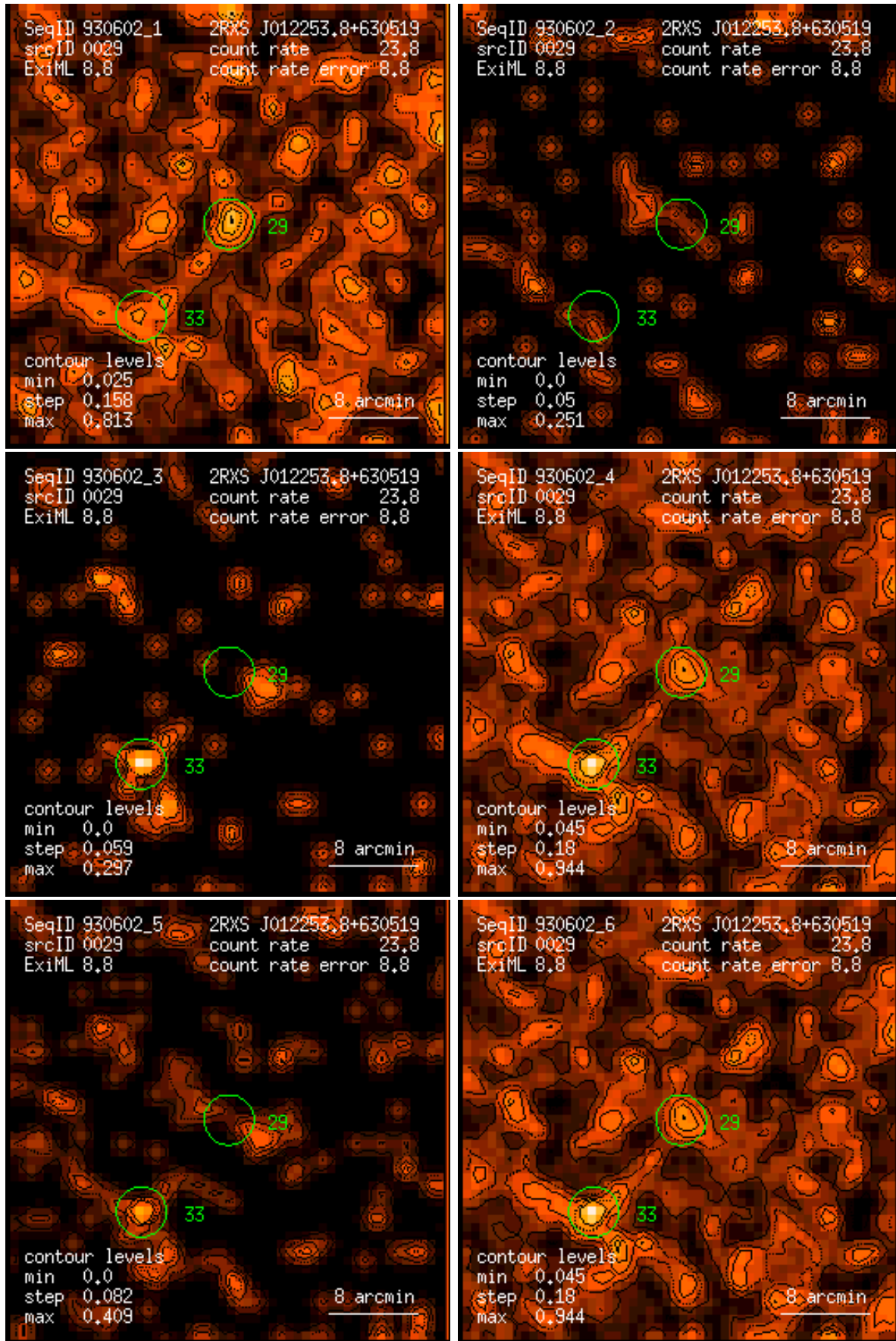
Figure 29: RASS 930602: detection 0029: band rate images, Gaussian filter: (1) PSPC channels 11 – 41, (2) 52 – 90, (3) 91 – 201, (4) 11 – 235, (5) 52 – 201, (6) 11 – 201. Broad band rates in counts/ks. Band rate contour levels in counts/ks/arcmin 2 .
