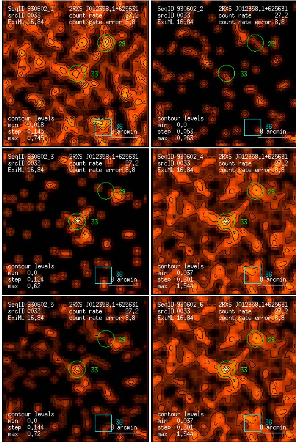
Figure 33: RASS 930602: detection 0033: band rate images, Gaussian filter: (1) PSPC channels 11 – 41, (2) 52 – 90, (3) 91 – 201, (4) 11 – 235, (5) 52 – 201, (6) 11 – 201. Broad band rates in counts/ks. Band rate contour levels in counts/ks/arcmin 2 .
