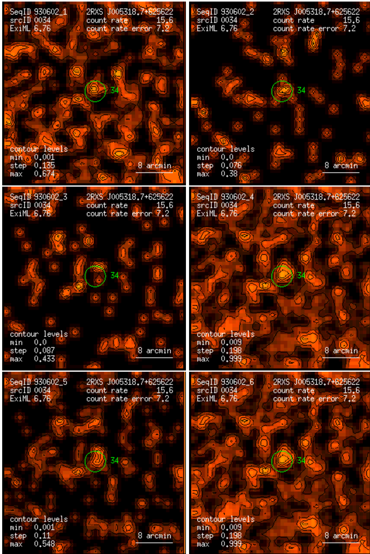
Figure 34: RASS 930602: detection 0034: band rate images, Gaussian filter: (1) PSPC channels 11 – 41, (2) 52 – 90, (3) 91 – 201, (4) 11 – 235, (5) 52 – 201, (6) 11 – 201. Broad band rates in counts/ks. Band rate contour levels in counts/ks/arcmin 2 .
