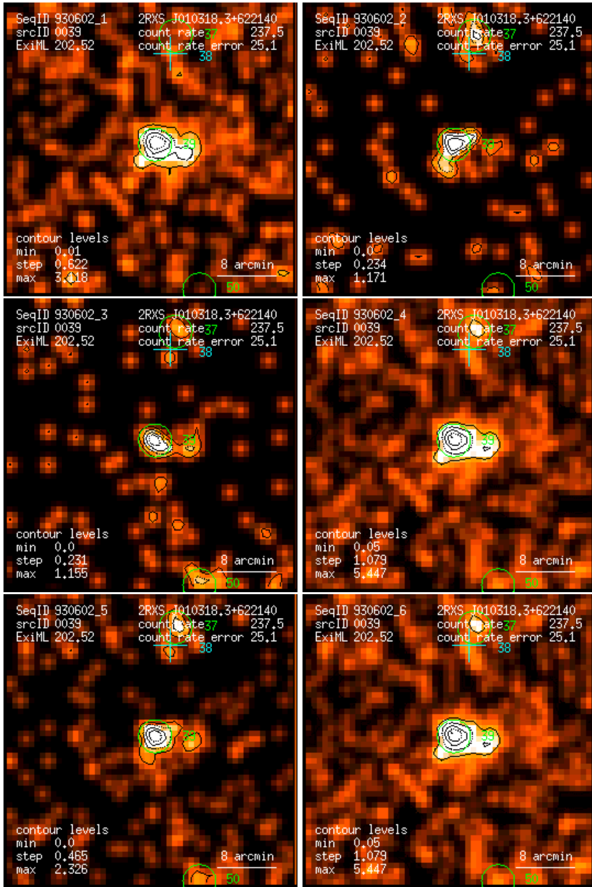
Figure 39: RASS 930602: detection 0039: band rate images, Gaussian filter: (1) PSPC channels 11 – 41, (2) 52 – 90, (3) 91 – 201, (4) 11 – 235, (5) 52 – 201, (6) 11 – 201. Broad band rates in counts/ks. Band rate contour levels in counts/ks/arcmin 2 .
