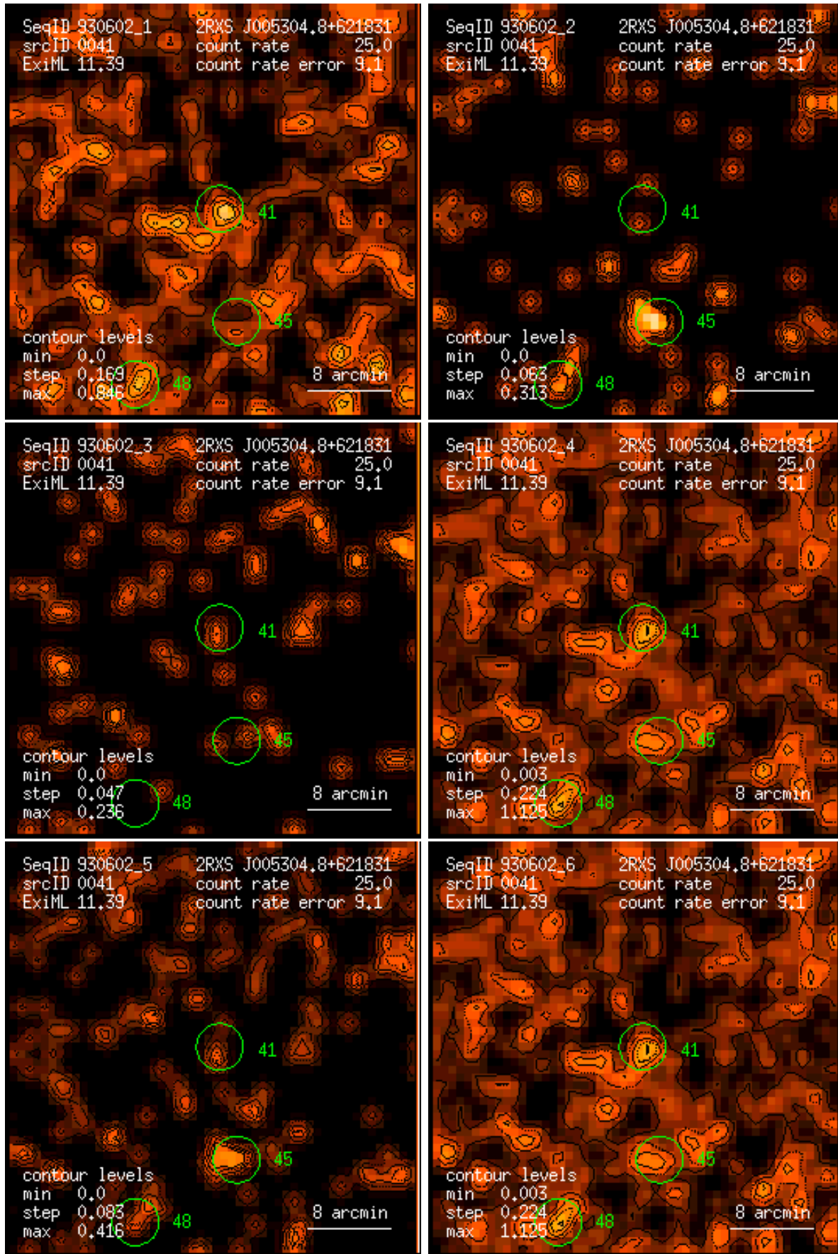
Figure 41: RASS 930602: detection 0041: band rate images, Gaussian filter: (1) PSPC channels 11 – 41, (2) 52 – 90, (3) 91 – 201, (4) 11 – 235, (5) 52 – 201, (6) 11 – 201. Broad band rates in counts/ks. Band rate contour levels in counts/ks/arcmin 2 .
