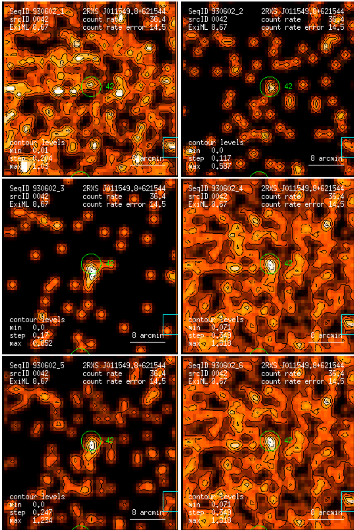
Figure 42: RASS 930602: detection 0042: band rate images, Gaussian filter: (1) PSPC channels 11 – 41, (2) 52 – 90, (3) 91 – 201, (4) 11 – 235, (5) 52 – 201, (6) 11 – 201. Broad band rates in counts/ks. Band rate contour levels in counts/ks/arcmin 2 .
