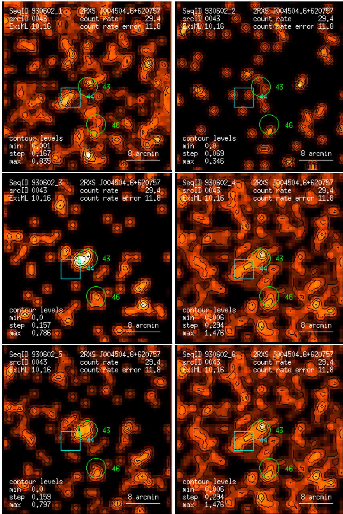
Figure 43: RASS 930602: detection 0043: band rate images, Gaussian filter: (1) PSPC channels 11 – 41, (2) 52 – 90, (3) 91 – 201, (4) 11 – 235, (5) 52 – 201, (6) 11 – 201. Broad band rates in counts/ks. Band rate contour levels in counts/ks/arcmin 2 .
