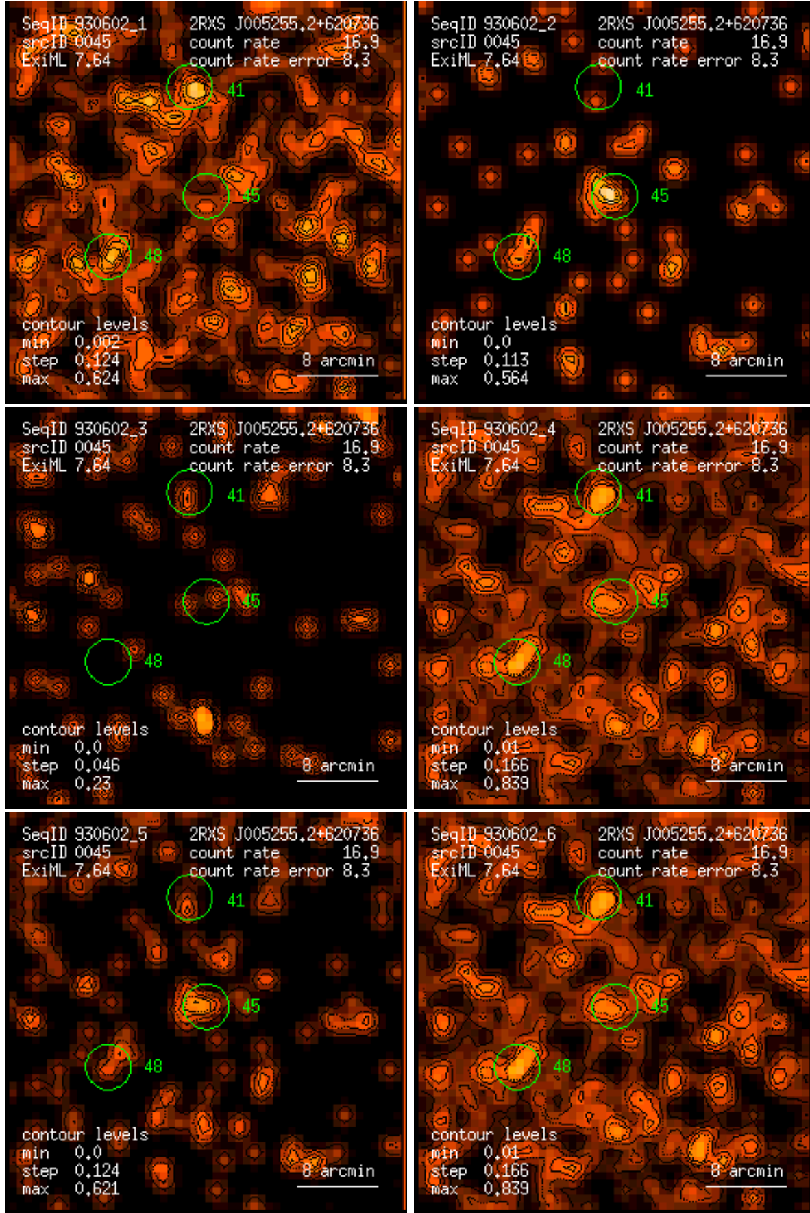
Figure 45: RASS 930602: detection 0045: band rate images, Gaussian filter: (1) PSPC channels 11 – 41, (2) 52 – 90, (3) 91 – 201, (4) 11 – 235, (5) 52 – 201, (6) 11 – 201. Broad band rates in counts/ks. Band rate contour levels in counts/ks/arcmin 2 .
