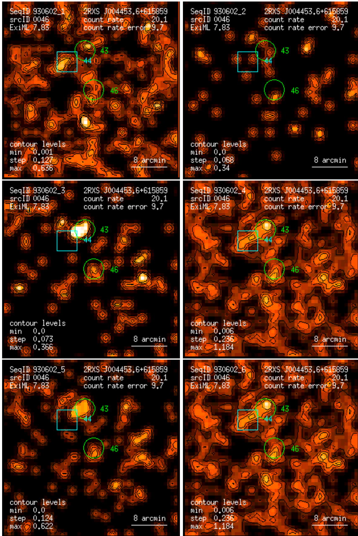
Figure 46: RASS 930602: detection 0046: band rate images, Gaussian filter: (1) PSPC channels 11 – 41, (2) 52 – 90, (3) 91 – 201, (4) 11 – 235, (5) 52 – 201, (6) 11 – 201. Broad band rates in counts/ks. Band rate contour levels in counts/ks/arcmin 2 .
