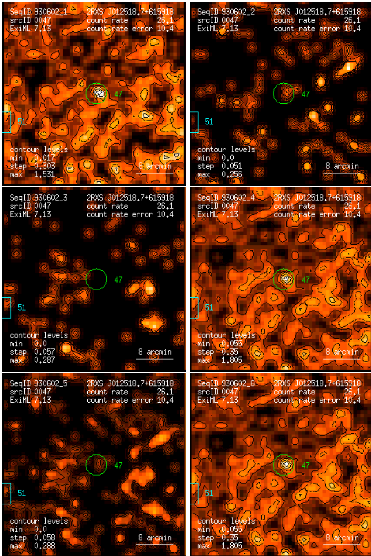
Figure 47: RASS 930602: detection 0047: band rate images, Gaussian filter: (1) PSPC channels 11 – 41, (2) 52 – 90, (3) 91 – 201, (4) 11 – 235, (5) 52 – 201, (6) 11 – 201. Broad band rates in counts/ks. Band rate contour levels in counts/ks/arcmin 2 .
