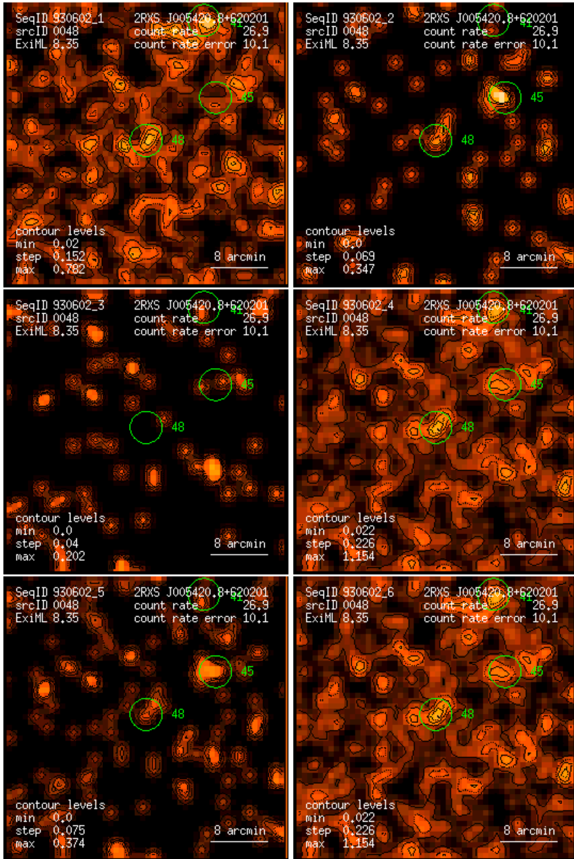
Figure 48: RASS 930602: detection 0048: band rate images, Gaussian filter: (1) PSPC channels 11 – 41, (2) 52 – 90, (3) 91 – 201, (4) 11 – 235, (5) 52 – 201, (6) 11 – 201. Broad band rates in counts/ks. Band rate contour levels in counts/ks/arcmin 2 .
