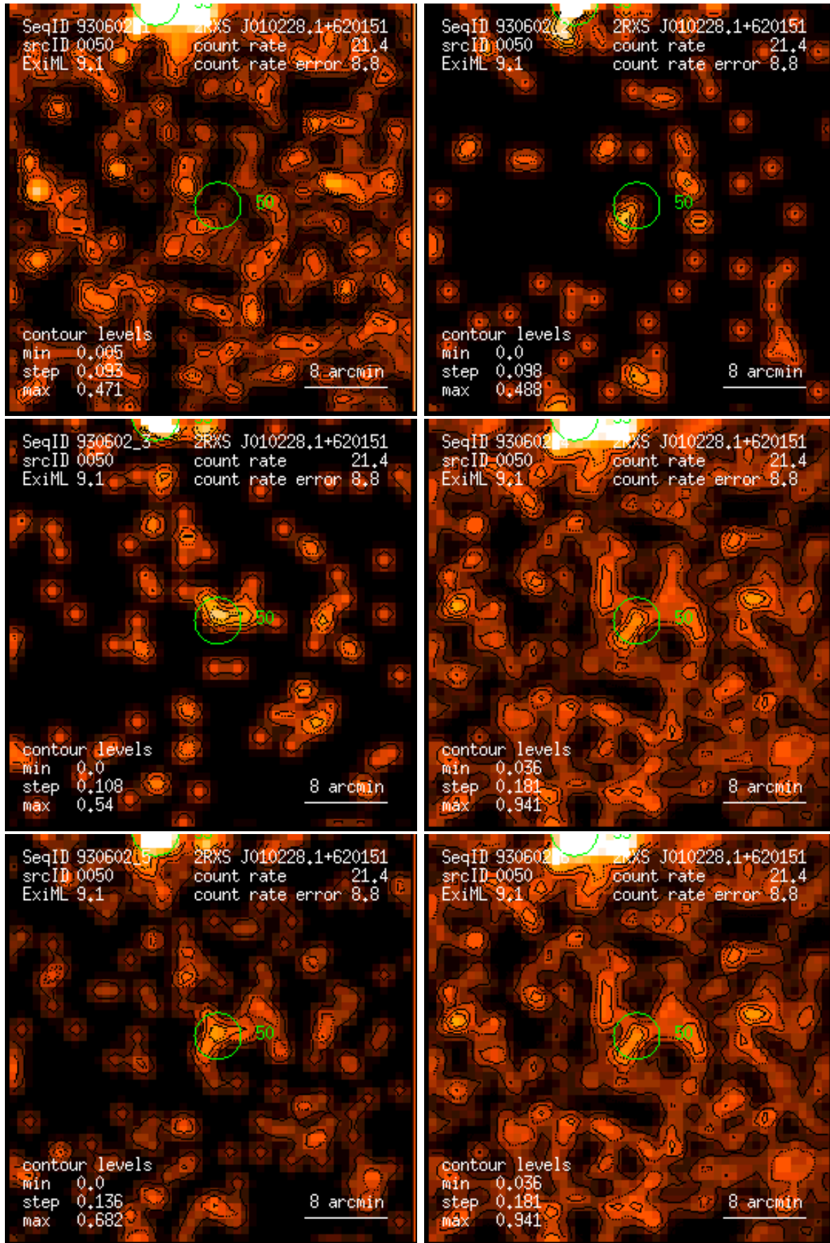
Figure 50: RASS 930602: detection 0050: band rate images, Gaussian filter: (1) PSPC channels 11 – 41, (2) 52 – 90, (3) 91 – 201, (4) 11 – 235, (5) 52 – 201, (6) 11 – 201. Broad band rates in counts/ks. Band rate contour levels in counts/ks/arcmin 2 .
