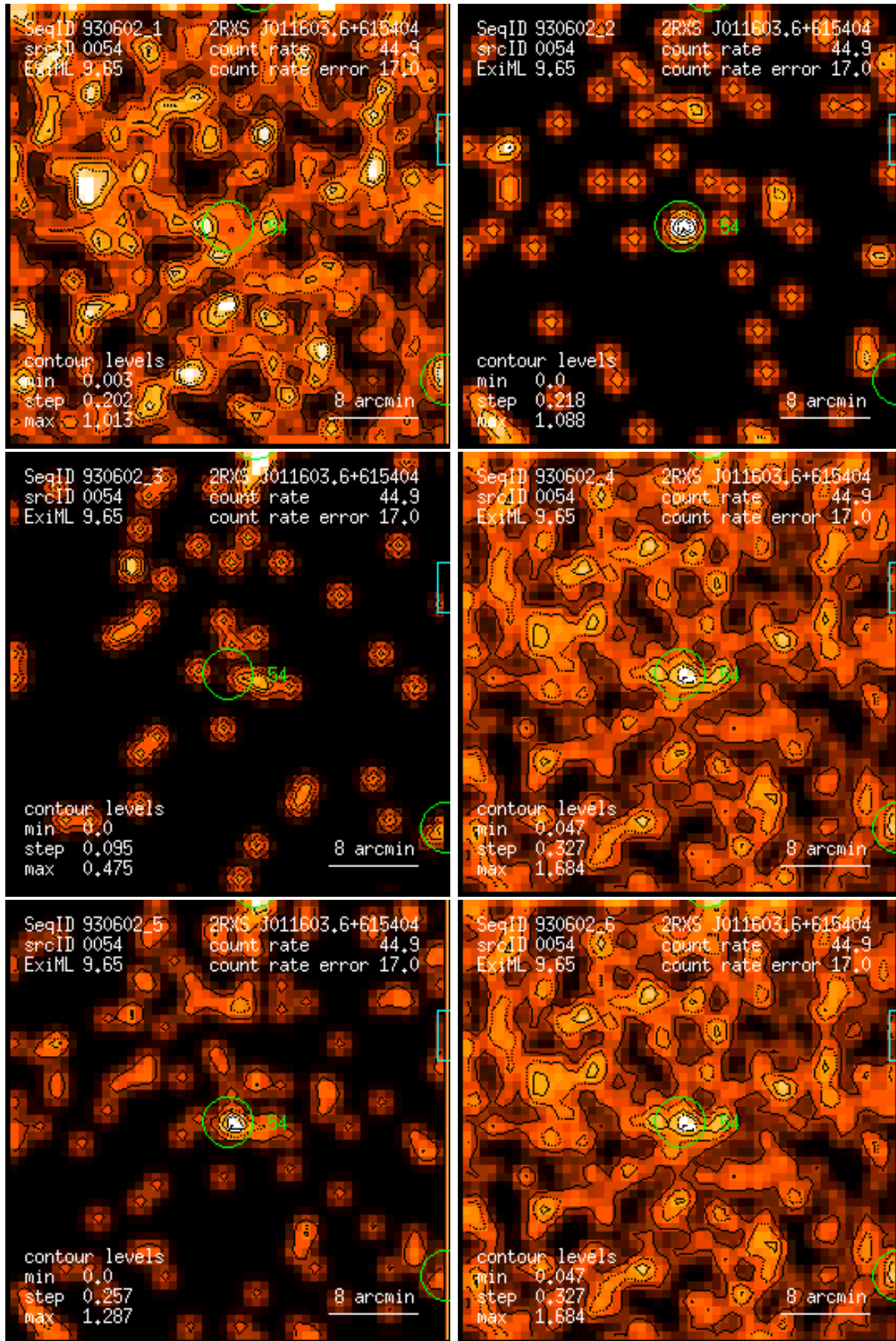
Figure 54: RASS 930602: detection 0054: band rate images, Gaussian filter: (1) PSPC channels 11 – 41, (2) 52 – 90, (3) 91 – 201, (4) 11 – 235, (5) 52 – 201, (6) 11 – 201. Broad band rates in counts/ks. Band rate contour levels in counts/ks/arcmin 2 .
