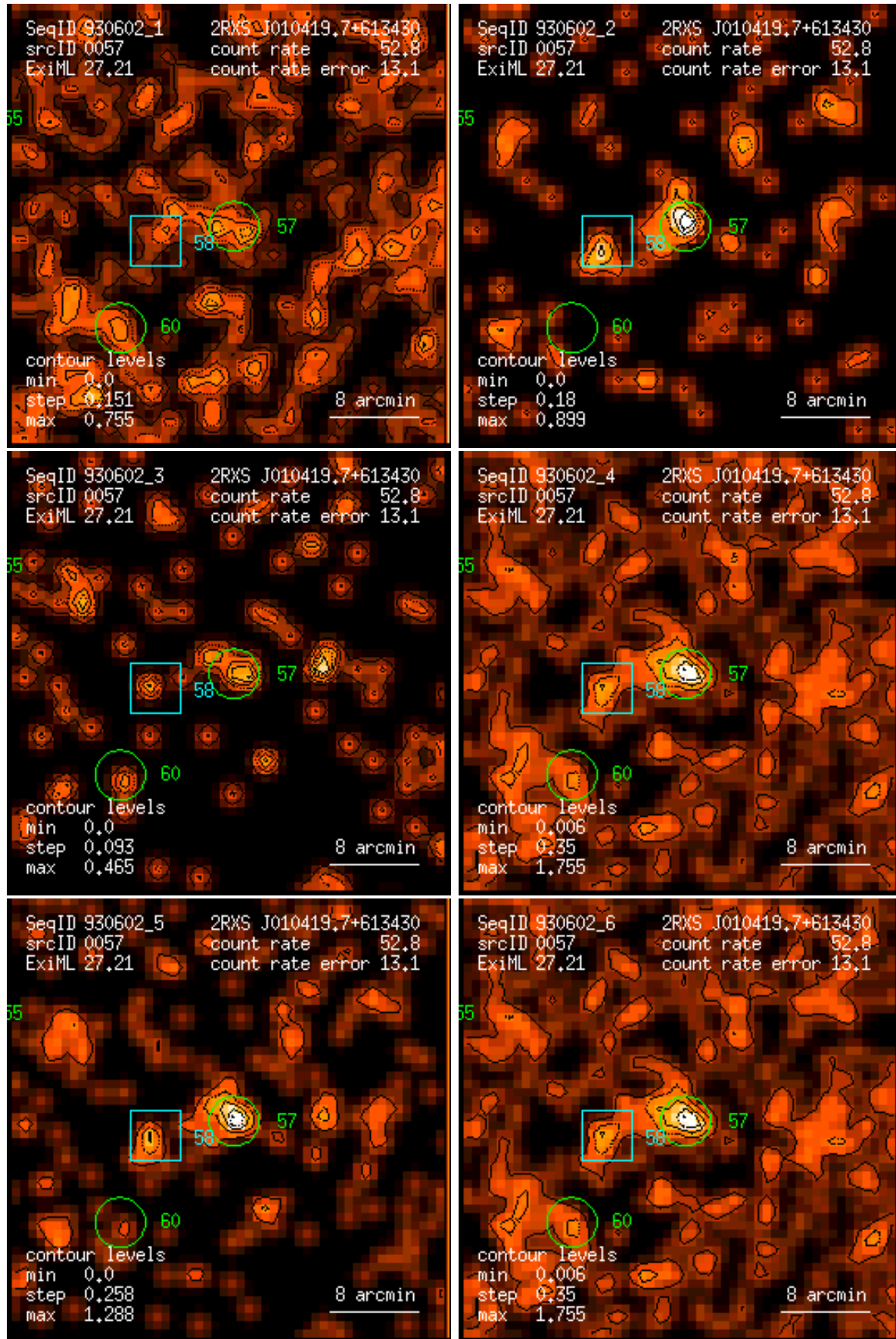
Figure 57: RASS 930602: detection 0057: band rate images, Gaussian filter: (1) PSPC channels 11 – 41, (2) 52 – 90, (3) 91 – 201, (4) 11 – 235, (5) 52 – 201, (6) 11 – 201. Broad band rates in counts/ks. Band rate contour levels in counts/ks/arcmin 2 .
