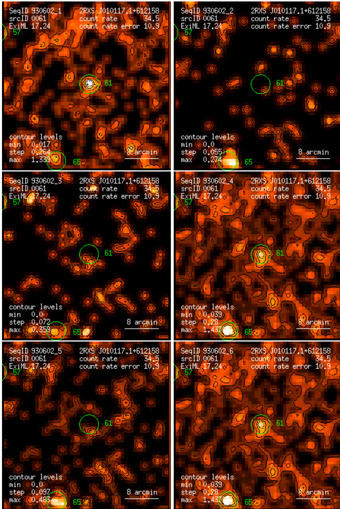
Figure 61: RASS 930602: detection 0061: band rate images, Gaussian filter: (1) PSPC channels 11 – 41, (2) 52 – 90, (3) 91 – 201, (4) 11 – 235, (5) 52 – 201, (6) 11 – 201. Broad band rates in counts/ks. Band rate contour levels in counts/ks/arcmin 2 .
