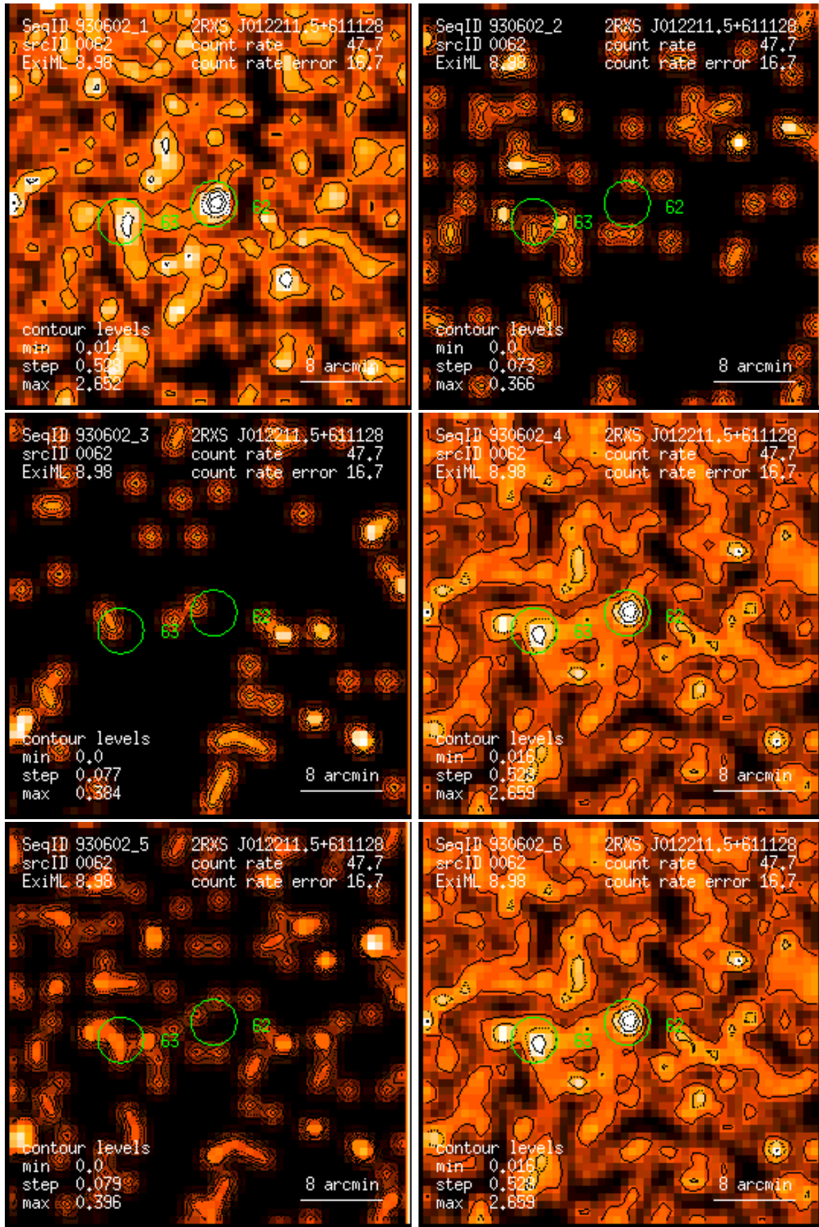
Figure 62: RASS 930602: detection 0062: band rate images, Gaussian filter: (1) PSPC channels 11 – 41, (2) 52 – 90, (3) 91 – 201, (4) 11 – 235, (5) 52 – 201, (6) 11 – 201. Broad band rates in counts/ks. Band rate contour levels in counts/ks/arcmin 2 .
