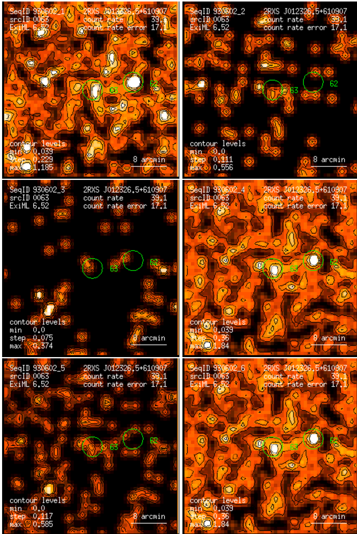
Figure 63: RASS 930602: detection 0063: band rate images, Gaussian filter: (1) PSPC channels 11 – 41, (2) 52 – 90, (3) 91 – 201, (4) 11 – 235, (5) 52 – 201, (6) 11 – 201. Broad band rates in counts/ks. Band rate contour levels in counts/ks/arcmin 2 .
