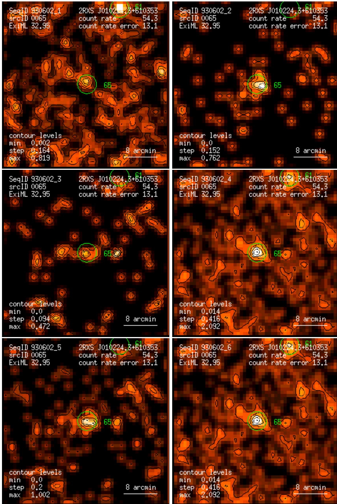
Figure 65: RASS 930602: detection 0065: band rate images, Gaussian filter: (1) PSPC channels 11 – 41, (2) 52 – 90, (3) 91 – 201, (4) 11 – 235, (5) 52 – 201, (6) 11 – 201. Broad band rates in counts/ks. Band rate contour levels in counts/ks/arcmin 2 .
