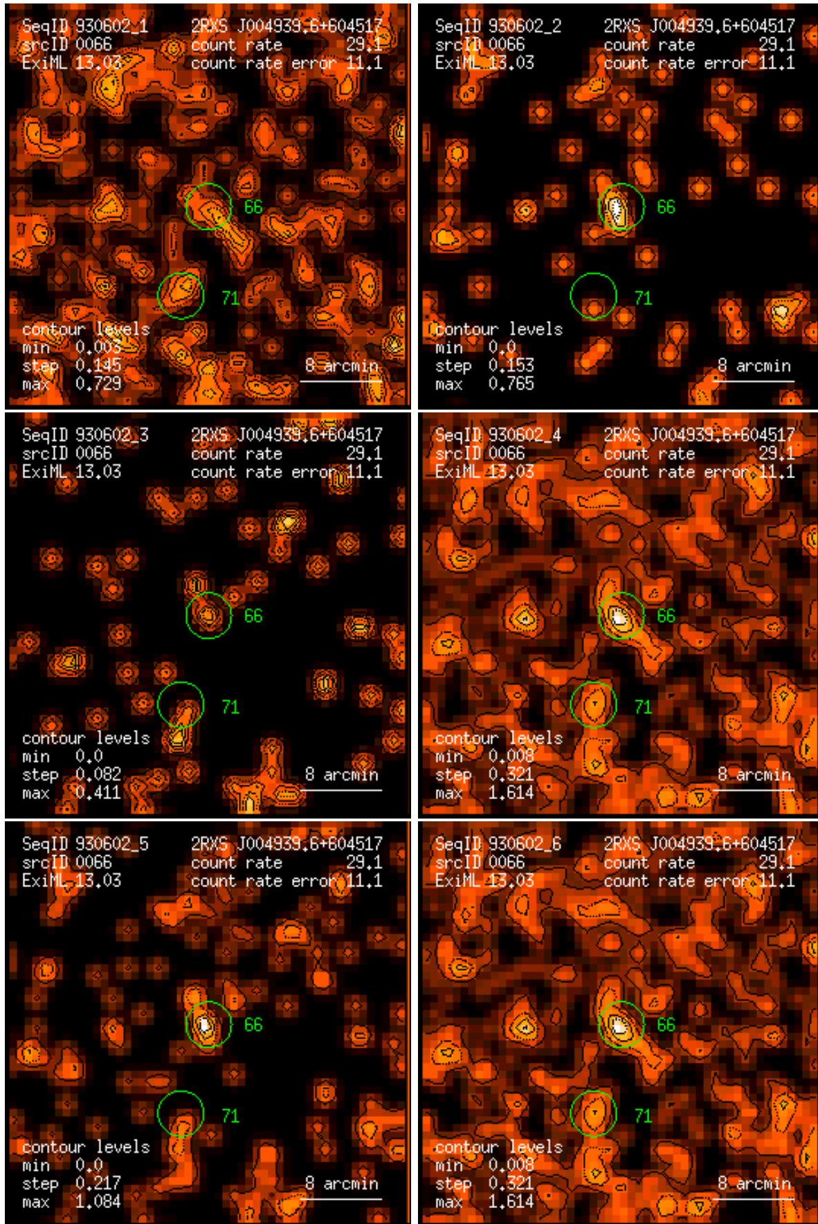
Figure 66: RASS 930602: detection 0066: band rate images, Gaussian filter: (1) PSPC channels 11 – 41, (2) 52 – 90, (3) 91 – 201, (4) 11 – 235, (5) 52 – 201, (6) 11 – 201. Broad band rates in counts/ks. Band rate contour levels in counts/ks/arcmin 2 .
