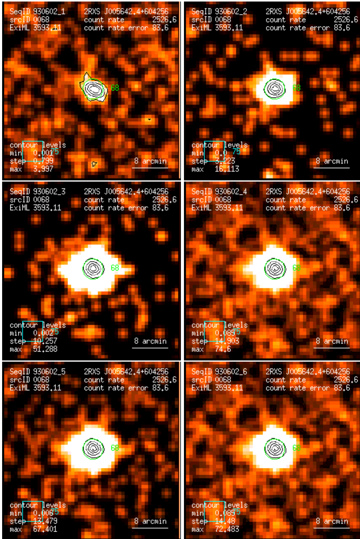
Figure 68: RASS 930602: detection 0068: band rate images, Gaussian filter: (1) PSPC channels 11 – 41, (2) 52 – 90, (3) 91 – 201, (4) 11 – 235, (5) 52 – 201, (6) 11 – 201. Broad band rates in counts/ks. Band rate contour levels in counts/ks/arcmin 2 .
