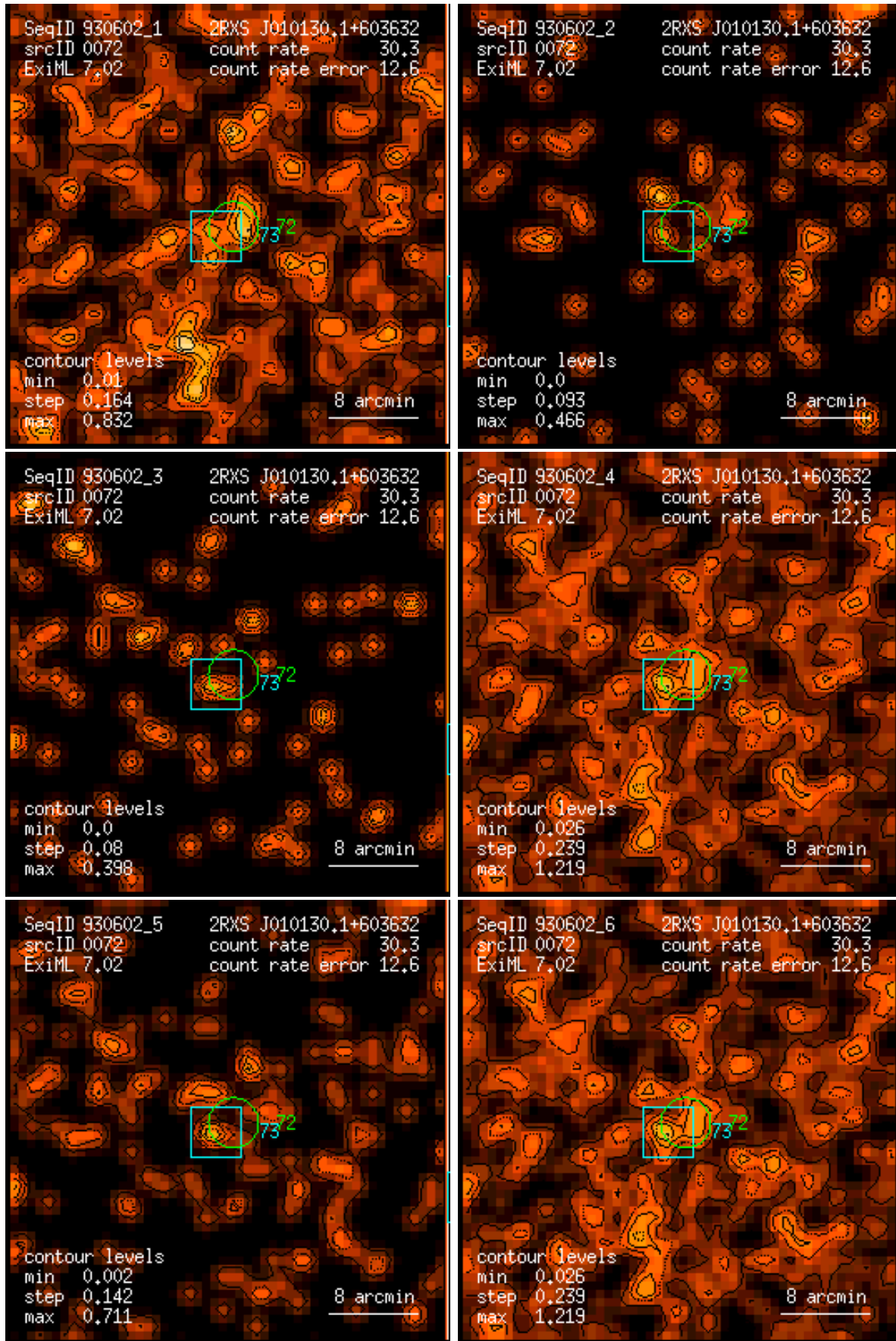
Figure 72: RASS 930602: detection 0072: band rate images, Gaussian filter: (1) PSPC channels 11 – 41, (2) 52 – 90, (3) 91 – 201, (4) 11 – 235, (5) 52 – 201, (6) 11 – 201. Broad band rates in counts/ks. Band rate contour levels in counts/ks/arcmin 2 .
