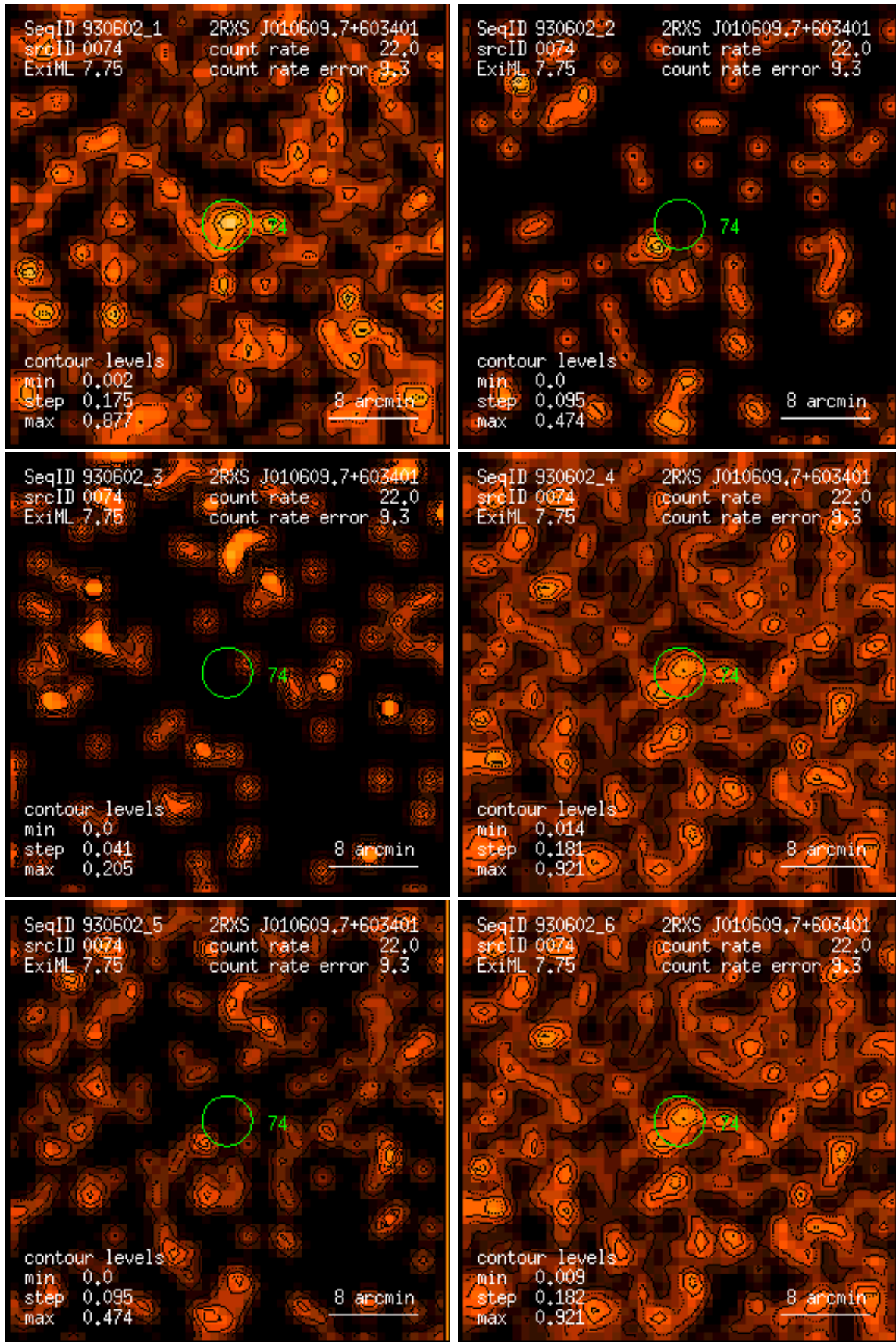
Figure 74: RASS 930602: detection 0074: band rate images, Gaussian filter: (1) PSPC channels 11 – 41, (2) 52 – 90, (3) 91 – 201, (4) 11 – 235, (5) 52 – 201, (6) 11 – 201. Broad band rates in counts/ks. Band rate contour levels in counts/ks/arcmin 2 .
