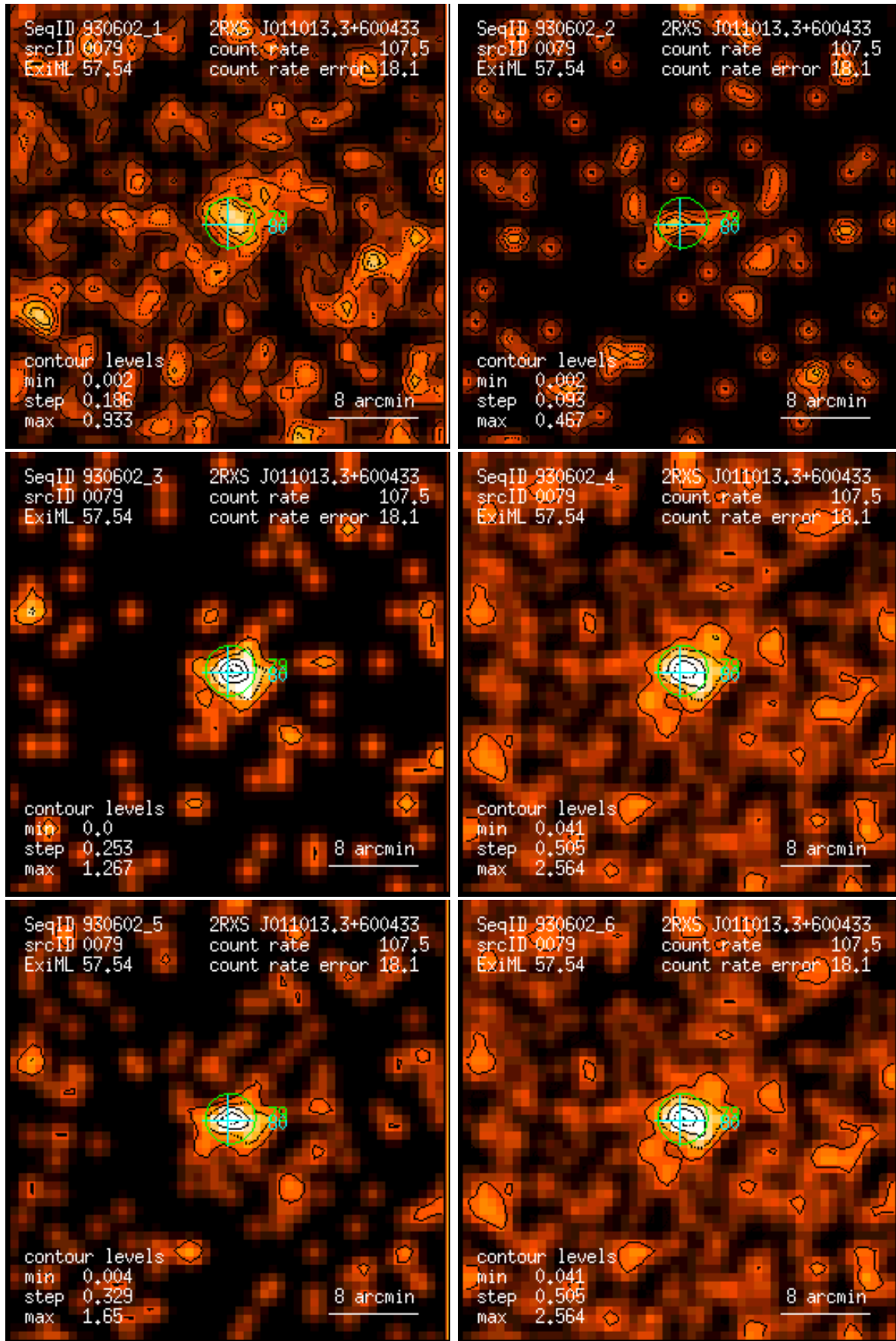
Figure 79: RASS 930602: detection 0079: band rate images, Gaussian filter: (1) PSPC channels 11 – 41, (2) 52 – 90, (3) 91 – 201, (4) 11 – 235, (5) 52 – 201, (6) 11 – 201. Broad band rates in counts/ks. Band rate contour levels in counts/ks/arcmin 2 .
