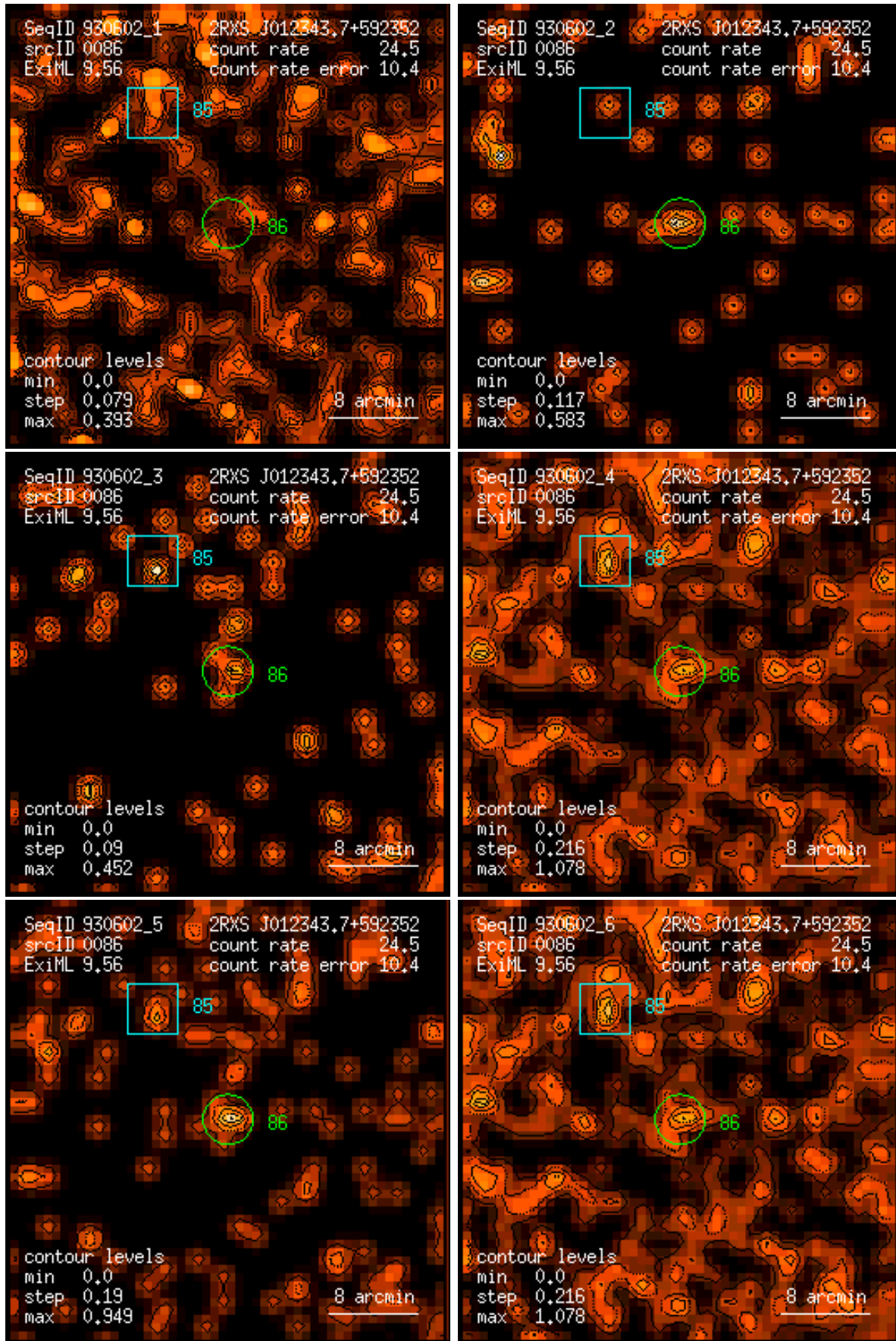
Figure 86: RASS 930602: detection 0086: band rate images, Gaussian filter: (1) PSPC channels 11 – 41, (2) 52 – 90, (3) 91 – 201, (4) 11 – 235, (5) 52 – 201, (6) 11 – 201. Broad band rates in counts/ks. Band rate contour levels in counts/ks/arcmin 2 .
