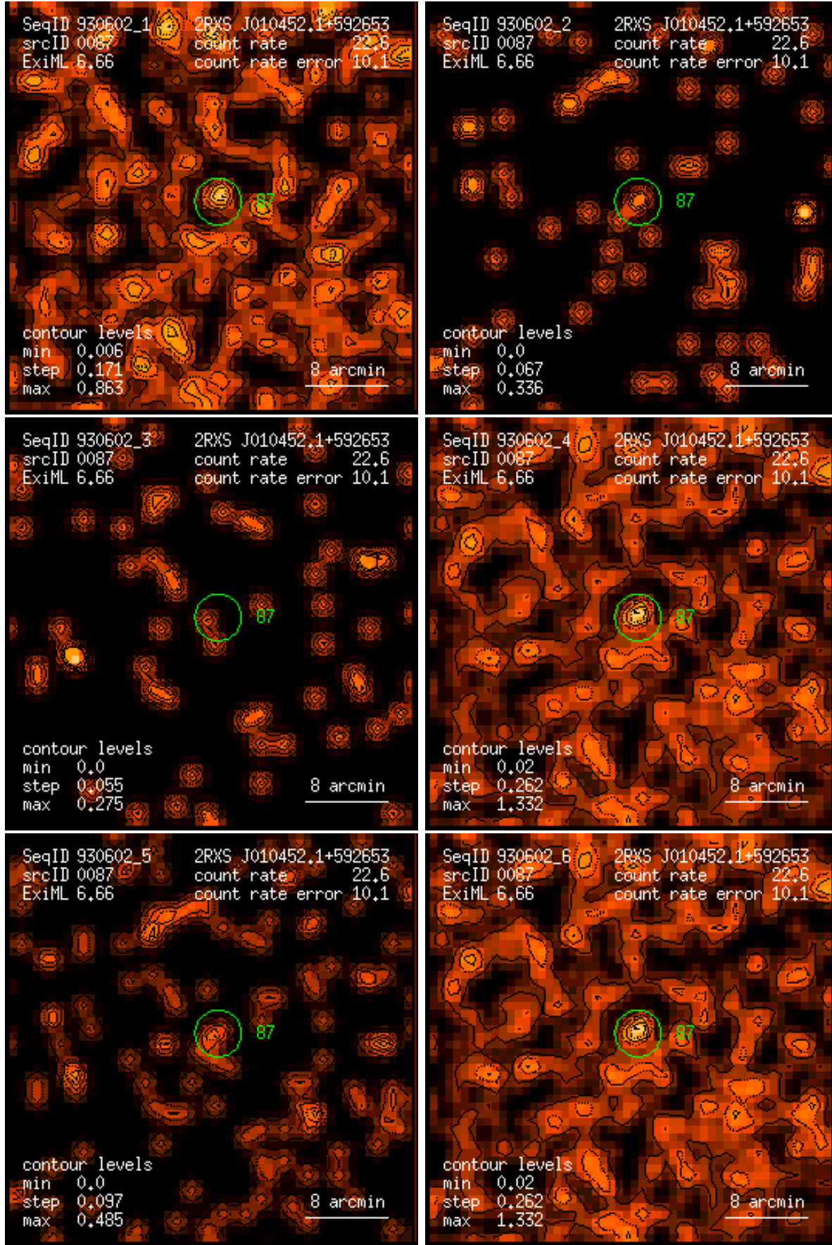
Figure 87: RASS 930602: detection 0087: band rate images, Gaussian filter: (1) PSPC channels 11 – 41, (2) 52 – 90, (3) 91 – 201, (4) 11 – 235, (5) 52 – 201, (6) 11 – 201. Broad band rates in counts/ks. Band rate contour levels in counts/ks/arcmin 2 .
