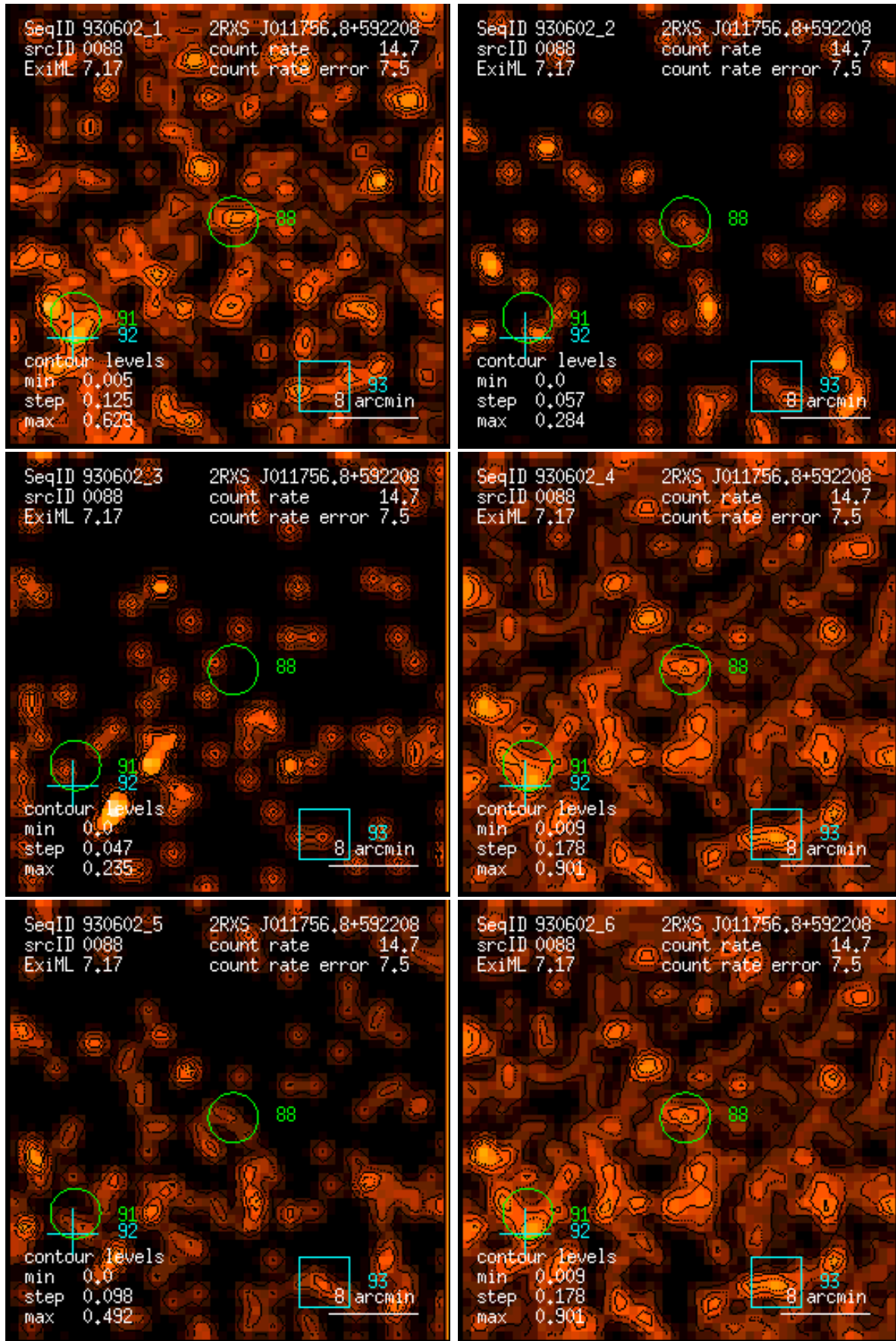
Figure 88: RASS 930602: detection 0088: band rate images, Gaussian filter: (1) PSPC channels 11 – 41, (2) 52 – 90, (3) 91 – 201, (4) 11 – 235, (5) 52 – 201, (6) 11 – 201. Broad band rates in counts/ks. Band rate contour levels in counts/ks/arcmin 2 .
