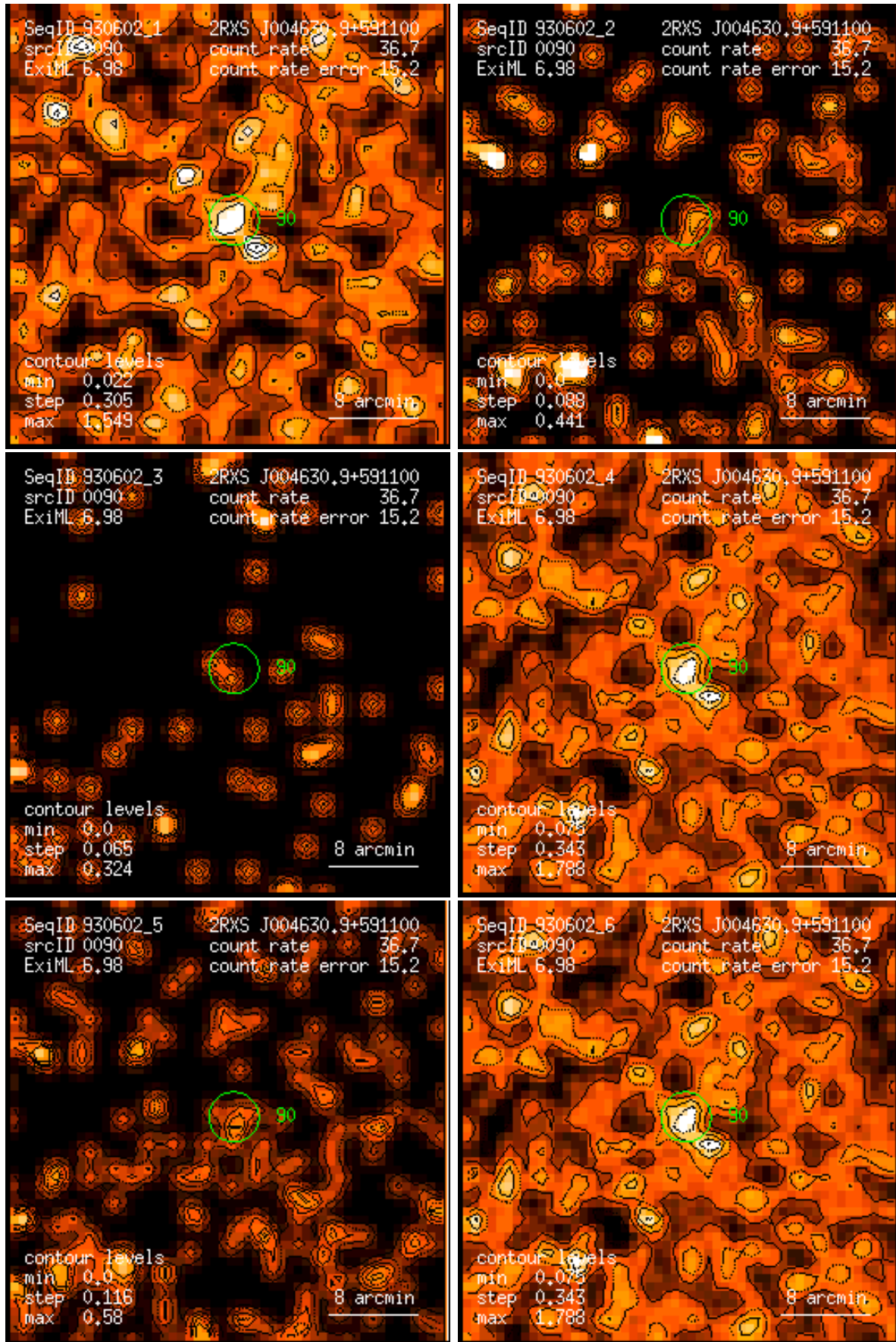
Figure 90: RASS 930602: detection 0090: band rate images, Gaussian filter: (1) PSPC channels 11 – 41, (2) 52 – 90, (3) 91 – 201, (4) 11 – 235, (5) 52 – 201, (6) 11 – 201. Broad band rates in counts/ks. Band rate contour levels in counts/ks/arcmin 2 .
