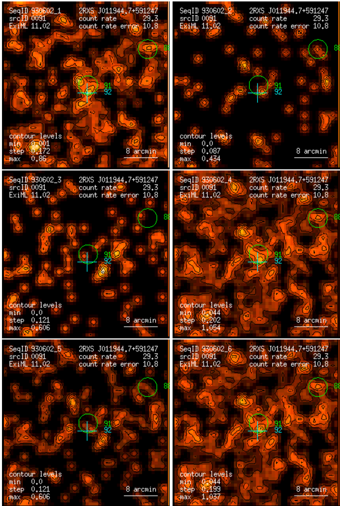
Figure 91: RASS 930602: detection 0091: band rate images, Gaussian filter: (1) PSPC channels 11 – 41, (2) 52 – 90, (3) 91 – 201, (4) 11 – 235, (5) 52 – 201, (6) 11 – 201. Broad band rates in counts/ks. Band rate contour levels in counts/ks/arcmin 2 .
