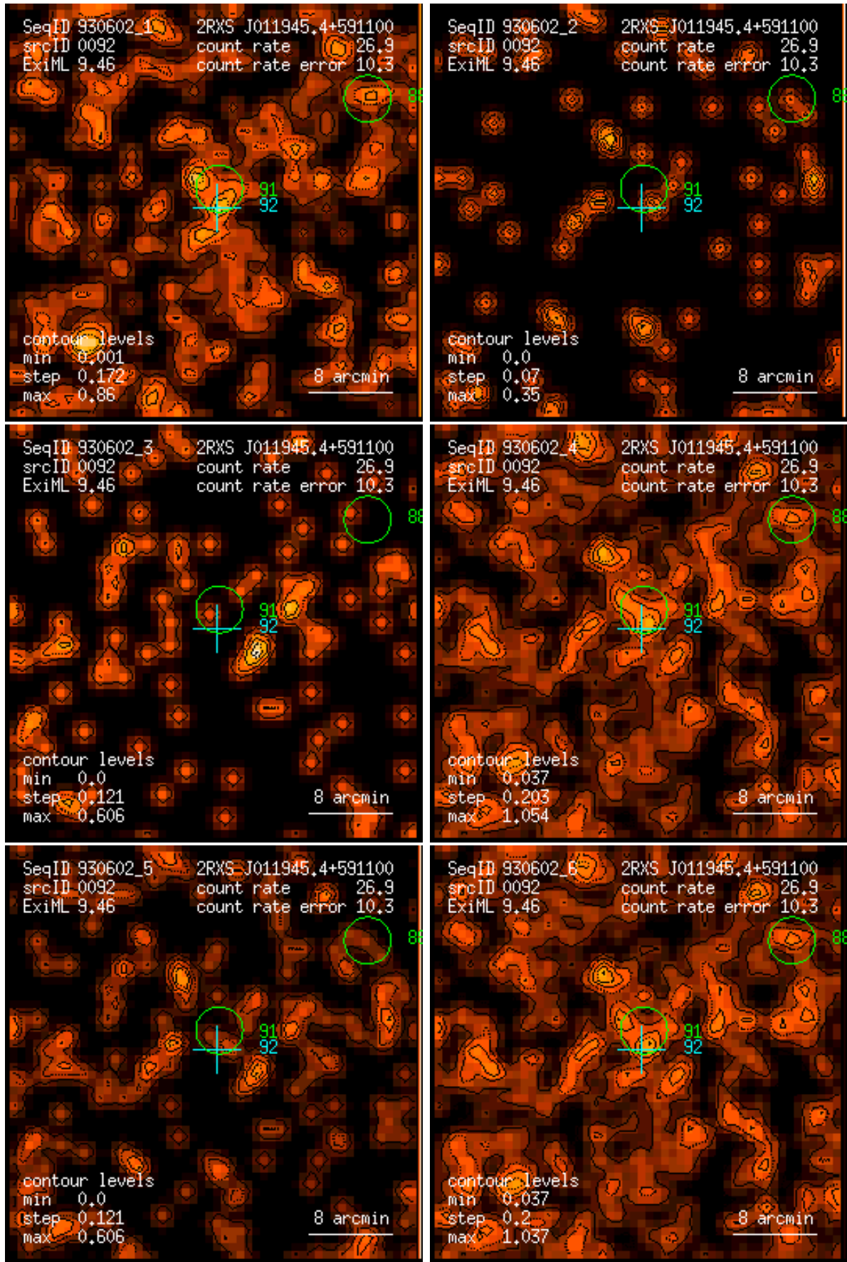
Figure 92: RASS 930602: detection 0092: band rate images, Gaussian filter: (1) PSPC channels 11 – 41, (2) 52 – 90, (3) 91 – 201, (4) 11 – 235, (5) 52 – 201, (6) 11 – 201. Broad band rates in counts/ks. Band rate contour levels in counts/ks/arcmin 2 .
