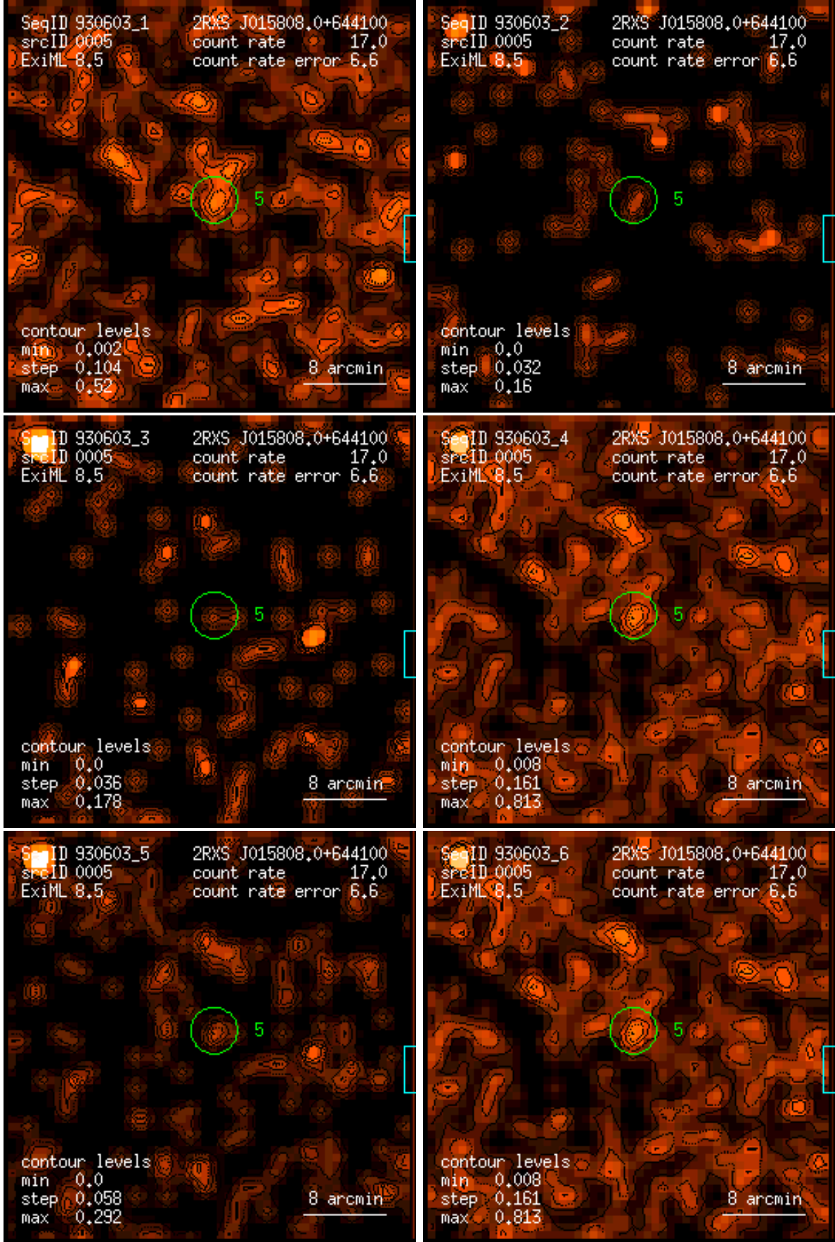
Figure 5: RASS 930603: detection 0005: band rate images, Gaussian filter: (1) PSPC channels 11 – 41, (2) 52 – 90, (3) 91 – 201, (4) 11 – 235, (5) 52 – 201, (6) 11 – 201. Broad band rates in counts/ks. Band rate contour levels in counts/ks/arcmin 2 .
