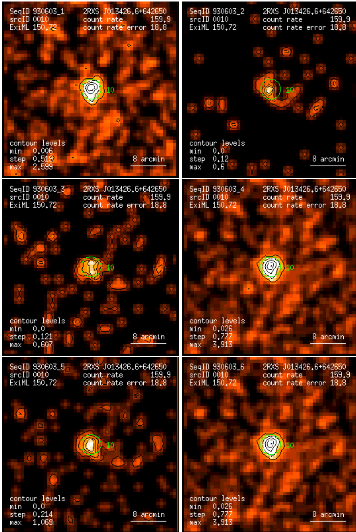
Figure 10: RASS 930603: detection 0010: band rate images, Gaussian filter: (1) PSPC channels 11 – 41, (2) 52 – 90, (3) 91 – 201, (4) 11 – 235, (5) 52 – 201, (6) 11 – 201. Broad band rates in counts/ks. Band rate contour levels in counts/ks/arcmin 2 .
