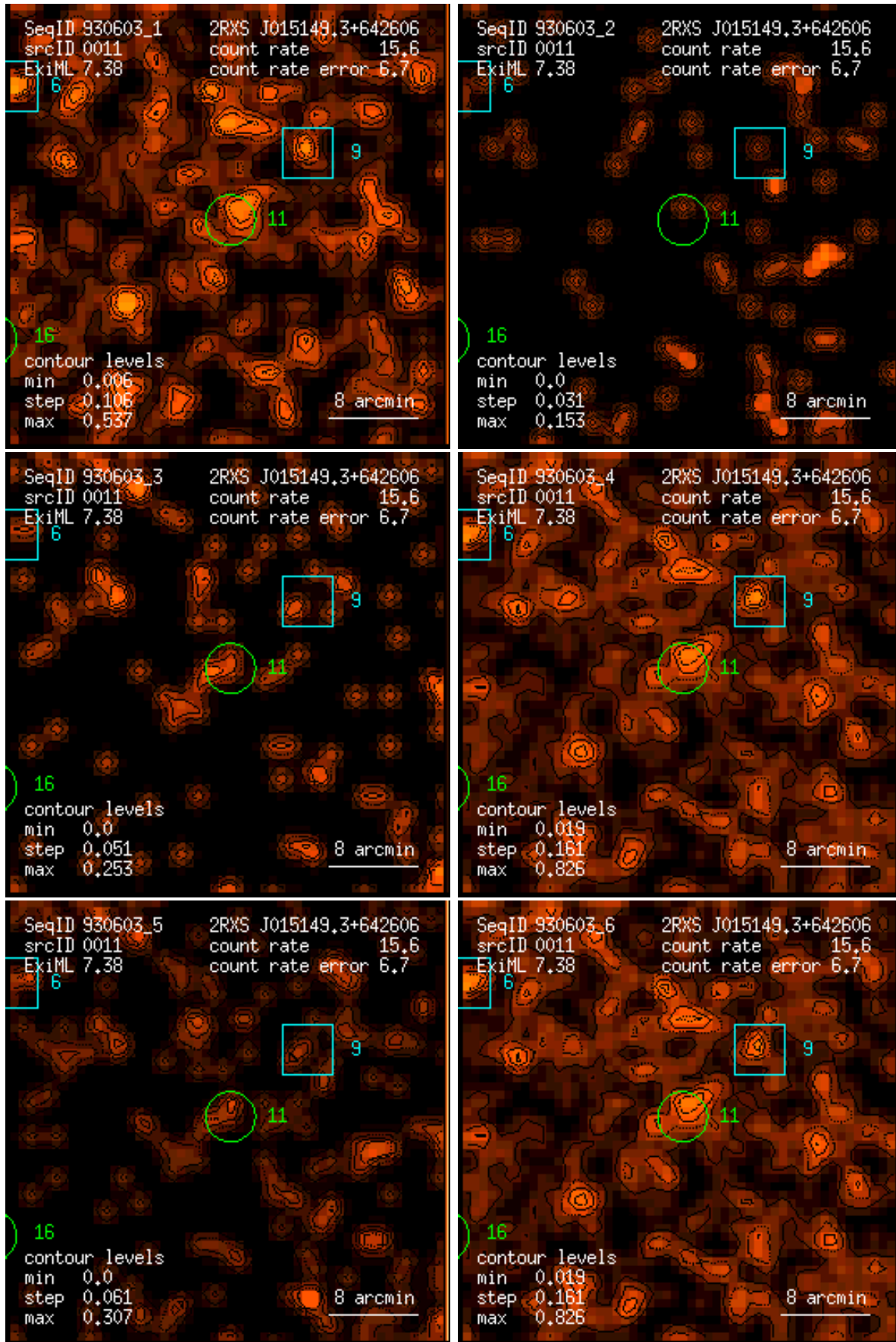
Figure 11: RASS 930603: detection 0011: band rate images, Gaussian filter: (1) PSPC channels 11 – 41, (2) 52 – 90, (3) 91 – 201, (4) 11 – 235, (5) 52 – 201, (6) 11 – 201. Broad band rates in counts/ks. Band rate contour levels in counts/ks/arcmin 2 .
