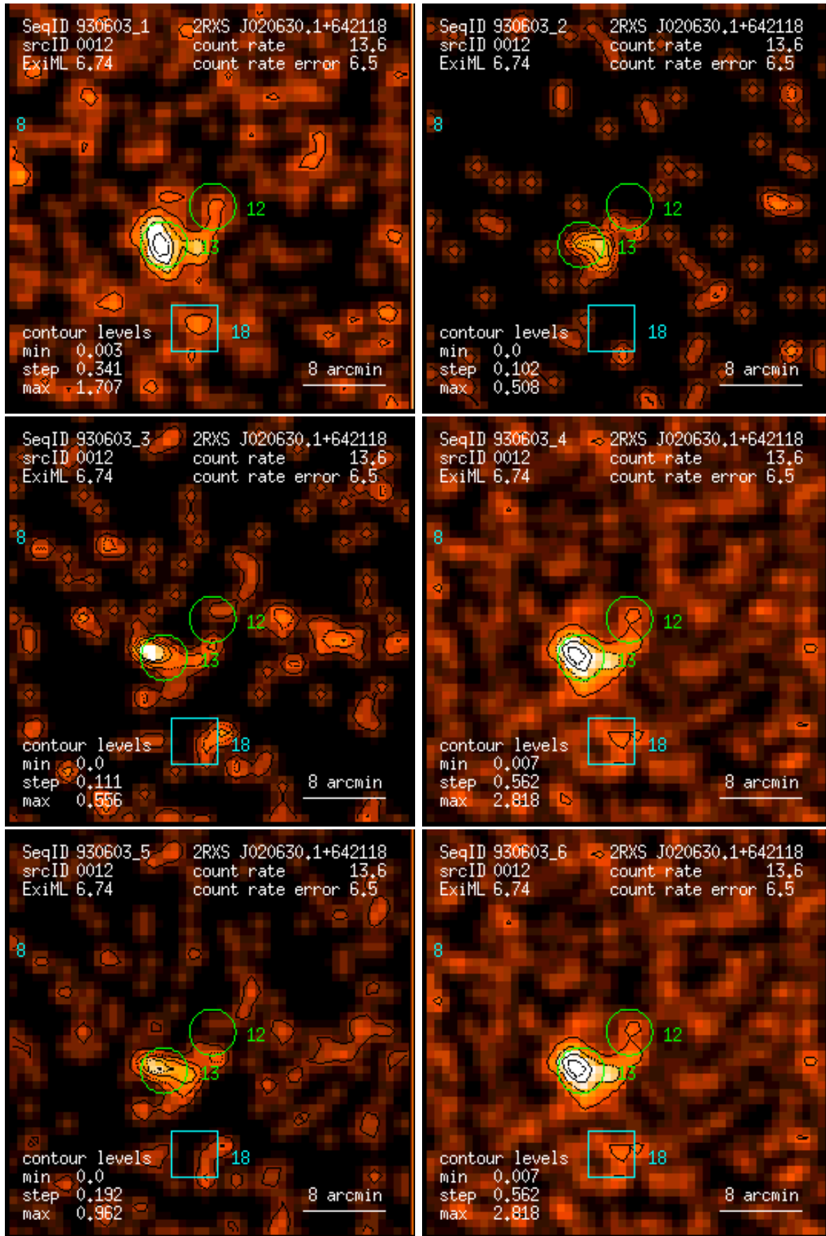
Figure 12: RASS 930603: detection 0012: band rate images, Gaussian filter: (1) PSPC channels 11 – 41, (2) 52 – 90, (3) 91 – 201, (4) 11 – 235, (5) 52 – 201, (6) 11 – 201. Broad band rates in counts/ks. Band rate contour levels in counts/ks/arcmin 2 .
