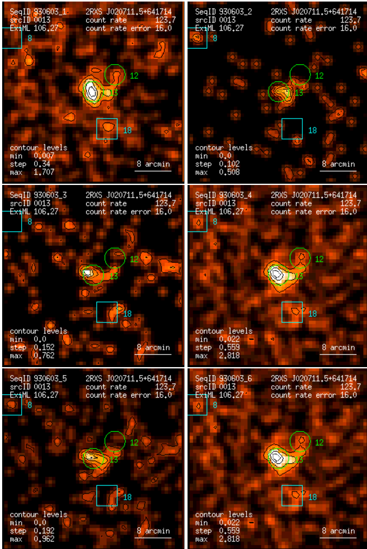
Figure 13: RASS 930603: detection 0013: band rate images, Gaussian filter: (1) PSPC channels 11 – 41, (2) 52 – 90, (3) 91 – 201, (4) 11 – 235, (5) 52 – 201, (6) 11 – 201. Broad band rates in counts/ks. Band rate contour levels in counts/ks/arcmin 2 .
