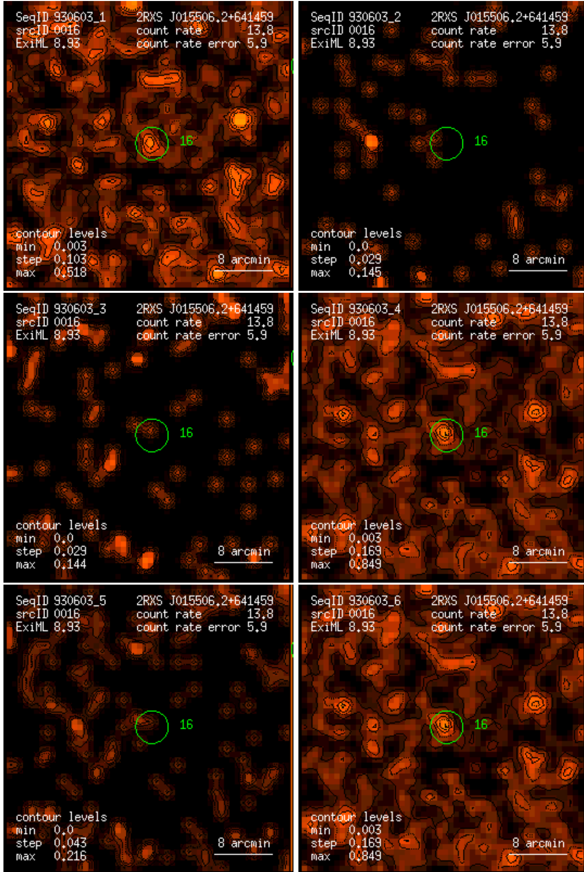
Figure 16: RASS 930603: detection 0016: band rate images, Gaussian filter: (1) PSPC channels 11 – 41, (2) 52 – 90, (3) 91 – 201, (4) 11 – 235, (5) 52 – 201, (6) 11 – 201. Broad band rates in counts/ks. Band rate contour levels in counts/ks/arcmin 2 .
