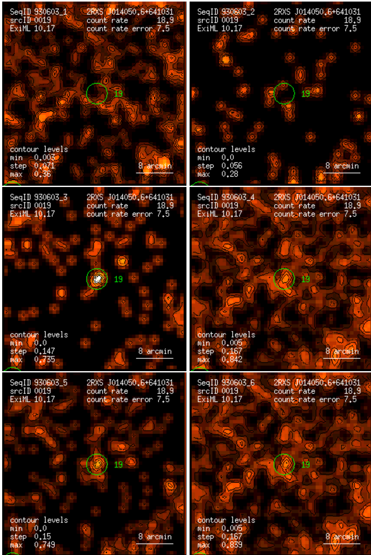
Figure 19: RASS 930603: detection 0019: band rate images, Gaussian filter: (1) PSPC channels 11 – 41, (2) 52 – 90, (3) 91 – 201, (4) 11 – 235, (5) 52 – 201, (6) 11 – 201. Broad band rates in counts/ks. Band rate contour levels in counts/ks/arcmin 2 .
