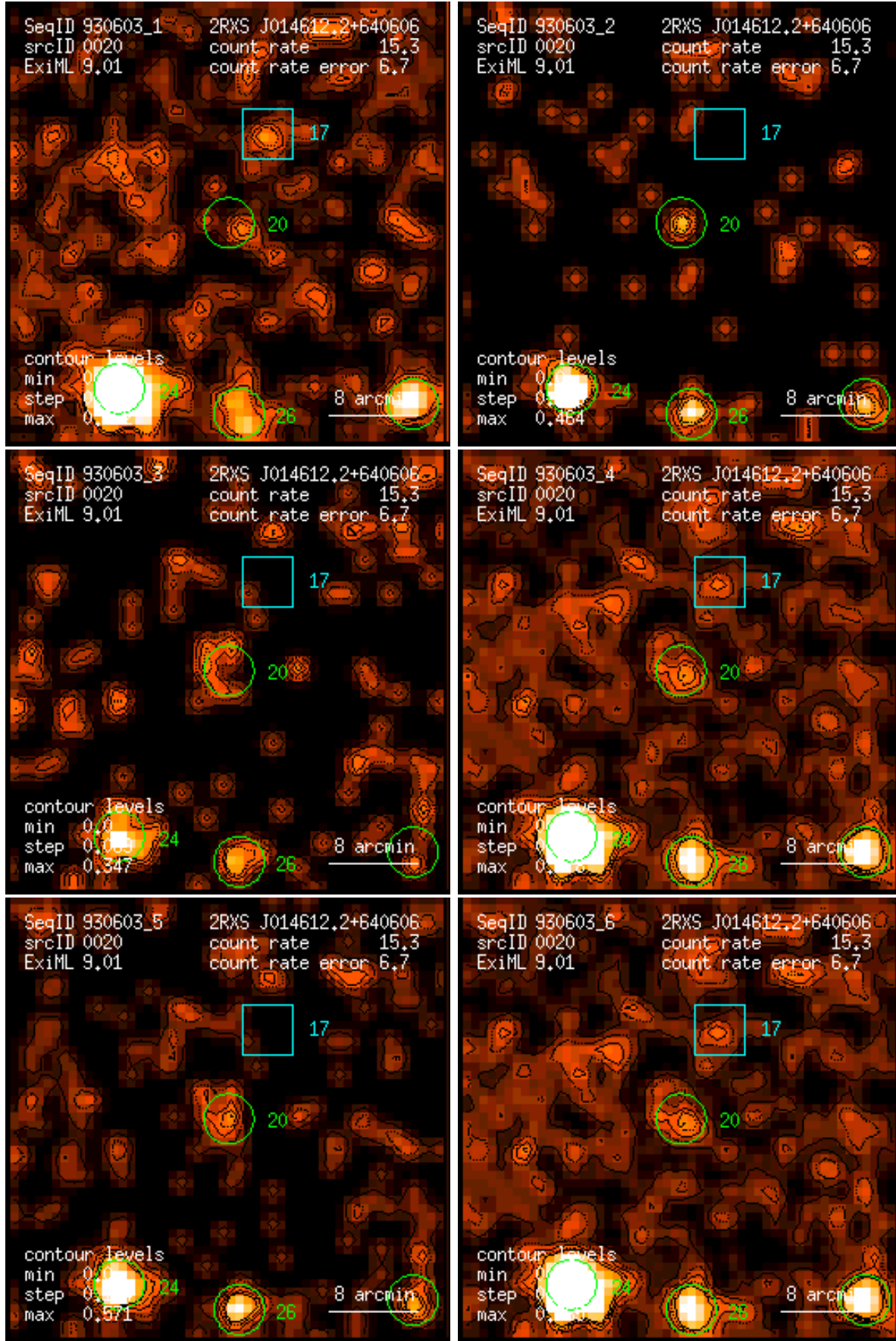
Figure 20: RASS 930603: detection 0020: band rate images, Gaussian filter: (1) PSPC channels 11 – 41, (2) 52 – 90, (3) 91 – 201, (4) 11 – 235, (5) 52 – 201, (6) 11 – 201. Broad band rates in counts/ks. Band rate contour levels in counts/ks/arcmin 2 .
