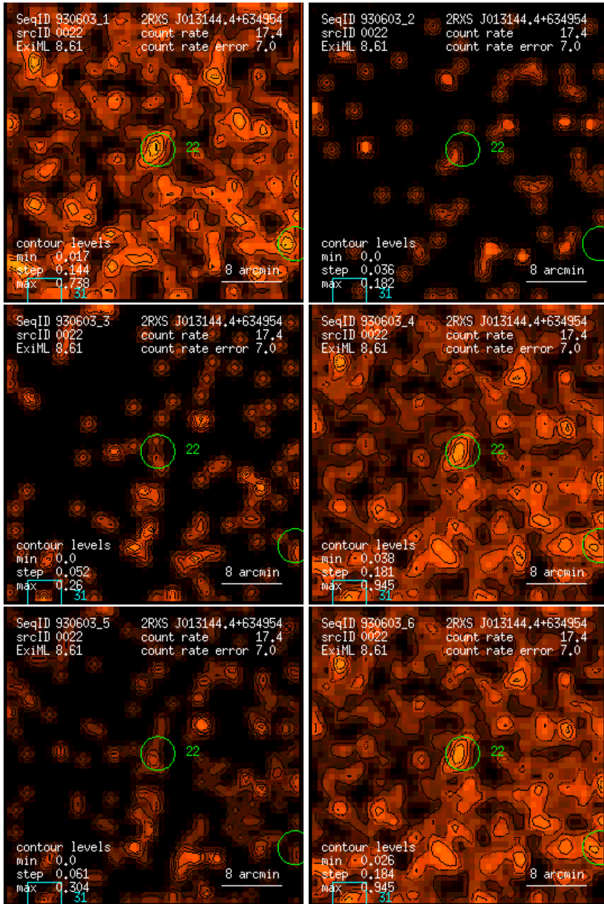
Figure 22: RASS 930603: detection 0022: band rate images, Gaussian filter: (1) PSPC channels 11 – 41, (2) 52 – 90, (3) 91 – 201, (4) 11 – 235, (5) 52 – 201, (6) 11 – 201. Broad band rates in counts/ks. Band rate contour levels in counts/ks/arcmin 2 .
